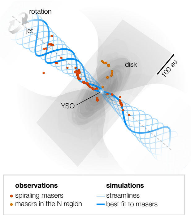
Fig. 1. Three-dimensional view of the MHD DW in IRAS 21078+5211 from simulations in Moscadelli et al. (2023). The observed maser positions (red and orange dots) are overlaid on streamlines (blue lines) computed from resistive-radiative-gravito-MHD simulations of a jet around a forming massive star.
