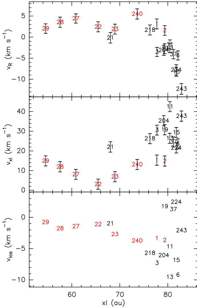
Fig. B.3: Distribution of velocities in the B2 stream. Maser labels (see Table 1) and error bars report values and corresponding errors for the velocity components along the R (upper panel), x_l (middle panel) and los (lower panel) axes. The error bars of the los components are not shown, as they are smaller than the labels. Red labels denote a subset of masers with similar velocity components.
