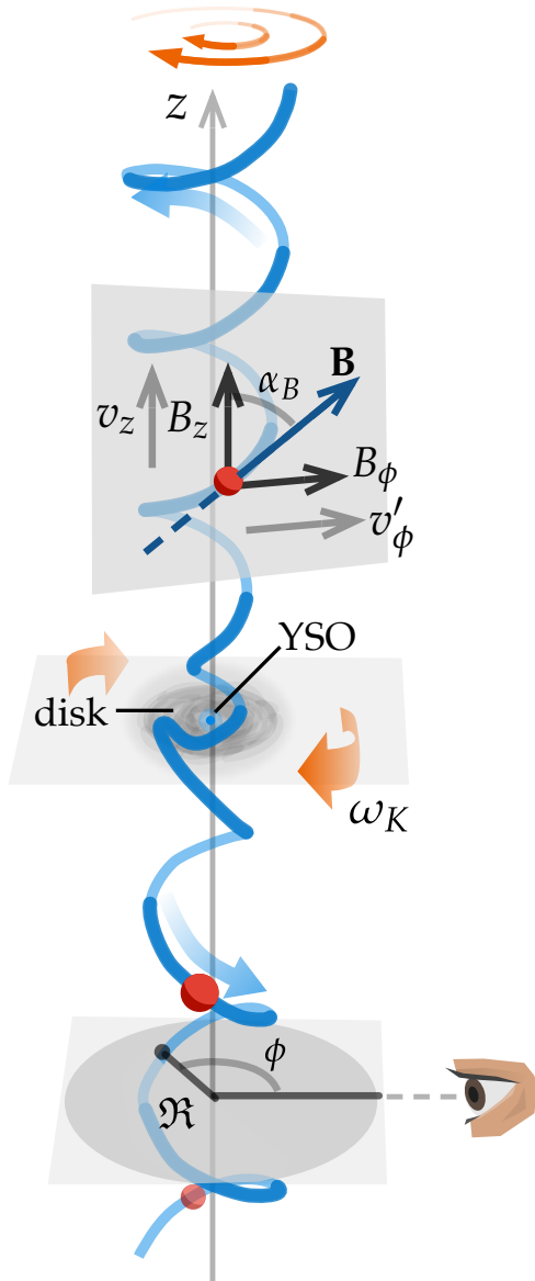
Fig. 6. Co-rotating helical magnetic field line. The water masers (red balls) move along a helical magnetic field line (blue) anchored to the rotating disk. The rotation radius and angle, \Re and \phi , and the axial, B_z and v_z , and azimuthal, B_\phi and v'_\phi , components of the magnetic field and velocity in the reference frame co-rotating with the disk are labeled. The tangent to the helix is inclined by an angle \alpha_B with respect to the z axis.
