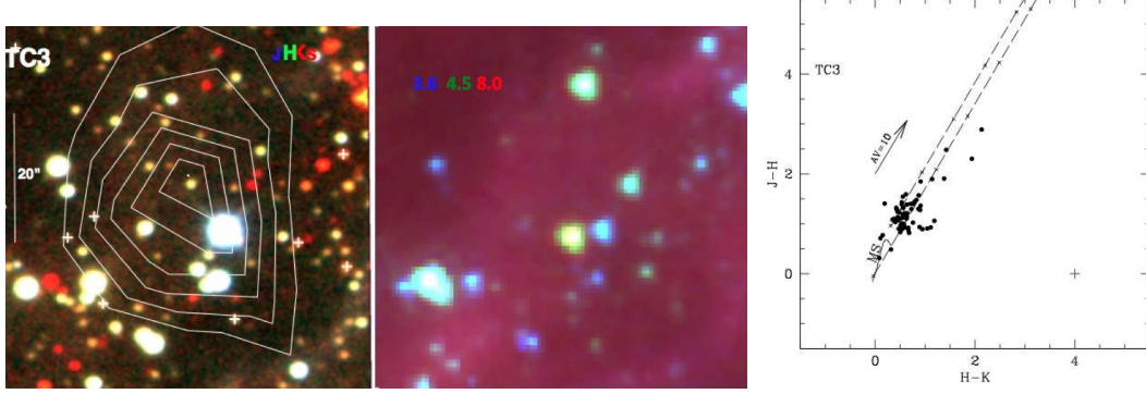
Figure 7: Left panel: JHK_s (blue, green, red) and IRAC/Spitzer true color images of a region of size 1' \times 1' around TC3. North is at the top and east to the left. Right panel: J-H versus H-K_s diagram of the near-IR sources observed in TC3.
