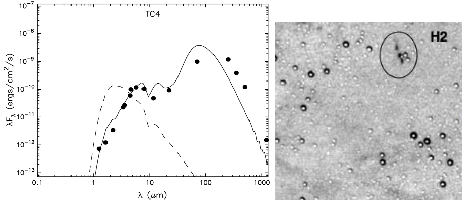
Figure 10: Left panel: Spectral energy distribution (SED) of TC4. The best-fit models of the SED derived from fitting tool [13] is over-plotted as solid line. Right panel: H_2 image of TC4.
