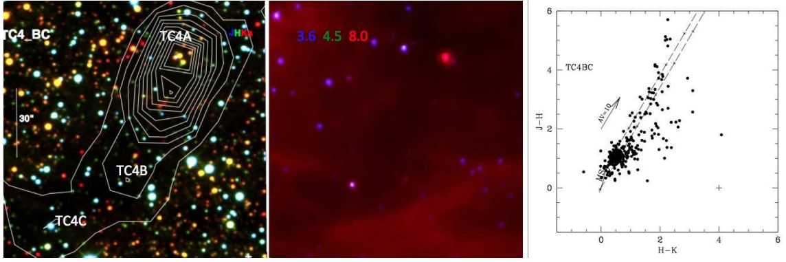
Figure 9: Left panel: JHK_s (blue, green, red) and IRAC/Spitzer true color images of a region of size 2' \times 2' around TC4. North is at the top and east to the left. Right panel: J-H versus H-K_s diagram of the near-IR sources observed in TC4.
