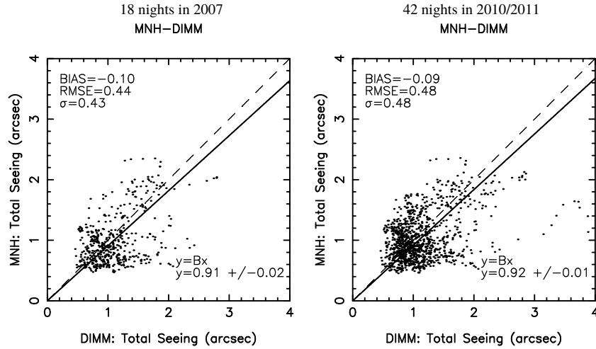
Figure 52: Scattered plot of the total seeing between Meso-NH outputs and DIMM measurements, for the summer periods of 2007, and 2010/2011. Both represent the validation sample.
