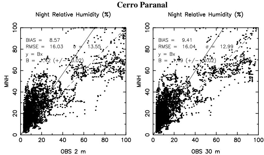
Figure 1: Scattered plot of Meso-NH relative humidity against observations, at 2 m and 30 m at Cerro Paranal , with the \Delta X = 500 m configuration. For the specific case of the relative humidity, 13 nights with very strong observed values for the RH (close to 100%), were added to the sample (for a total of 142 nights) of the simulated nights.
