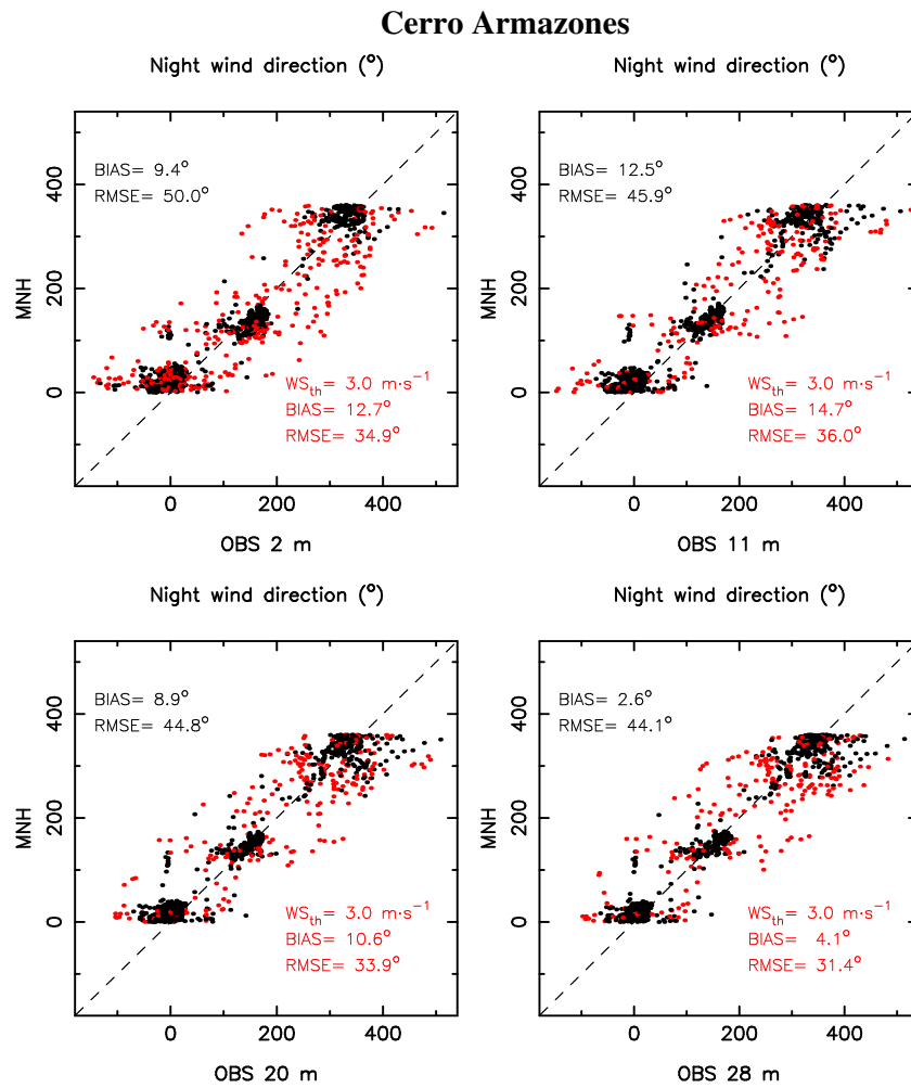
Figure 5: Scattered plot of Meso-NH wind direction against observations, at 2 m, 11 m, 20 m and 28 m at Cerro Armazones , with the \Delta X = 500 m configuration.
