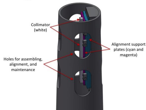
Fig. 7. Sketch of the parabolic segmented grazing-incidence mirror mounted on the tower.
