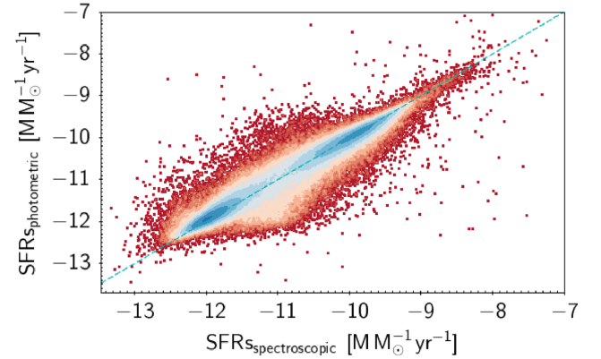
Figure 3. \text{SFR}_{\text{spectroscopic}} versus \text{SFR}_{\text{photometric}} scatter plot related to the MLPQNA _{\Phi\text{LAB}} experiment, selected to produce the final SFR catalogue (see Appendix B).
