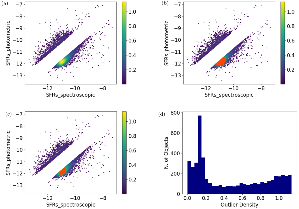
Figure 6. The scatter plot in the top left corner (a) shows the distribution of outliers in the \text{SFRs}_{\text{spectroscopic}} versus \text{SFRs}_{\text{photometric}} space with a superimposed density map, while the diagrams in the top right (b) and bottom left (c) corners show highlighted in orange all the objects with a density, respectively, six and eight times higher than the average point density. The histogram in the bottom right corner (d) shows the outliers density distribution.
