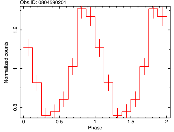
Figure 1. Pulse profile of XTE J1810–197 in the 1–6 keV range obtained in the XMM-Newton observation 0804590201. The pulse profiles of all the other 2017–2018 observations are very similar. They can be well described by a single sinusoid with average pulsed fraction of \sim 30 per cent.
