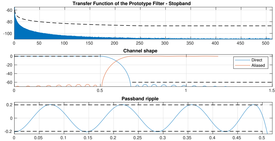
Figure 11. Theoretic filter response for the channelizer prototype filter
