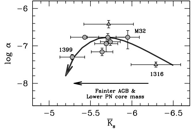
FIG. 8.— Luminosity-specific PN number ( \alpha ) vs. effective K luminosity for the galaxy sample of Table 2. The triangles mark galaxies with K_s inferred from F160W (see footnote 6). Note that a fainter AGB roughly correlates with a scantier PN stellar population among old/metal-rich (UV-enhanced) ellipticals, as expected from the long post-AGB to PN nucleus transition time, combined with the (shorter) evaporation timescale of the ejecta (compare the sketch on the plot with Fig. 15 of Buzzoni et al. 2006). A correspondingly low PN rate per unit galaxy luminosity is also to be expected, on the other hand, for younger stellar populations, as in the case of NGC 1316, as a consequence of higher stellar masses and a reduced PN nuclear lifetime. [See the electronic edition of the Journal for a color version of this figure.]
