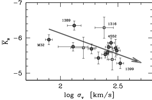
FIG. 7.— Absolute fluctuation magnitudes vs. velocity dispersion for the galaxy sample of Table 2. Squares mark galaxies with K_s extrapolated from F160W, as explained in footnote 6. [See the electronic edition of the Journal for a color version of this figure.]
