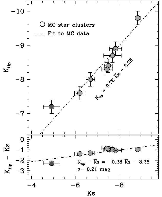
FIG. 3.—Absolute K_{tip} vs. \overline{K}_s magnitude relationship for Magellanic Cloud star clusters. Circles locate the average position for each “supercluster” of Table 1, i.e., a co-addition of several individual systems belonging to homogenous Searle et al. (1980) age classes. The dashed line is the fit to the data, as displayed on the plot. Color code for markers is the same as in Fig. 2. [See the electronic edition of the Journal for a color version of this figure.]
