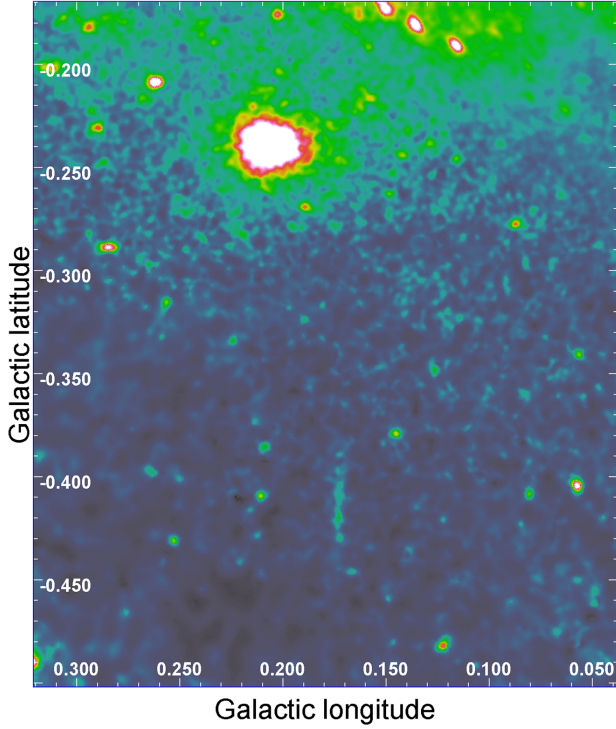
Figure 17. XMM–Newton image in the 2–12 keV band showing the new X-ray filament located south of the Radio Arc. The filament is located at l \simeq 0^\circ 173 and b \simeq -0^\circ 413 and appears as a thin ( <0.15 arcmin) and long ( \sim 2.7 arcmin) filament running along the north–south direction, as the Radio Arc. The brightest source in the image is SAX J1747.7–2853.
