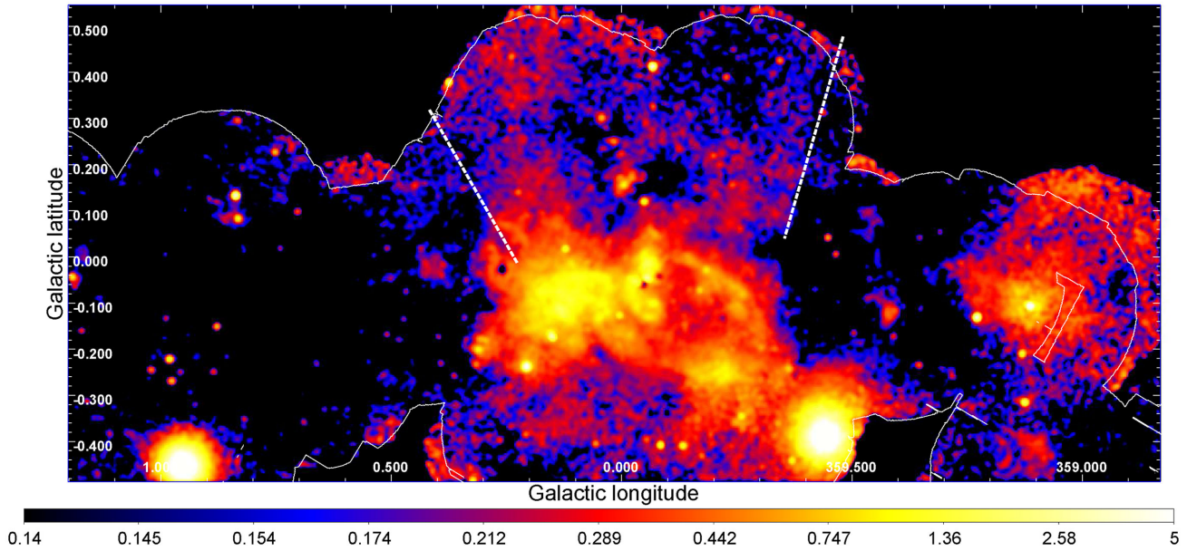
Figure 16. Map of the normalization of the soft thermal gas component (in units of 10^{-4} times the APEC normalization). The white lines indicate the extent of the survey having more than 7.2 ks exposure. The white dashed lines show the position of the two sharp edges in the distribution of the high-latitude plasma. Some bright point sources (i.e. 1E 1743.1–2843, AX J1745.6–2901, 1E 1740.7–2942, GRS 1741.9–2853) have been removed, thereby producing artificial holes in the maps at their respective locations.
