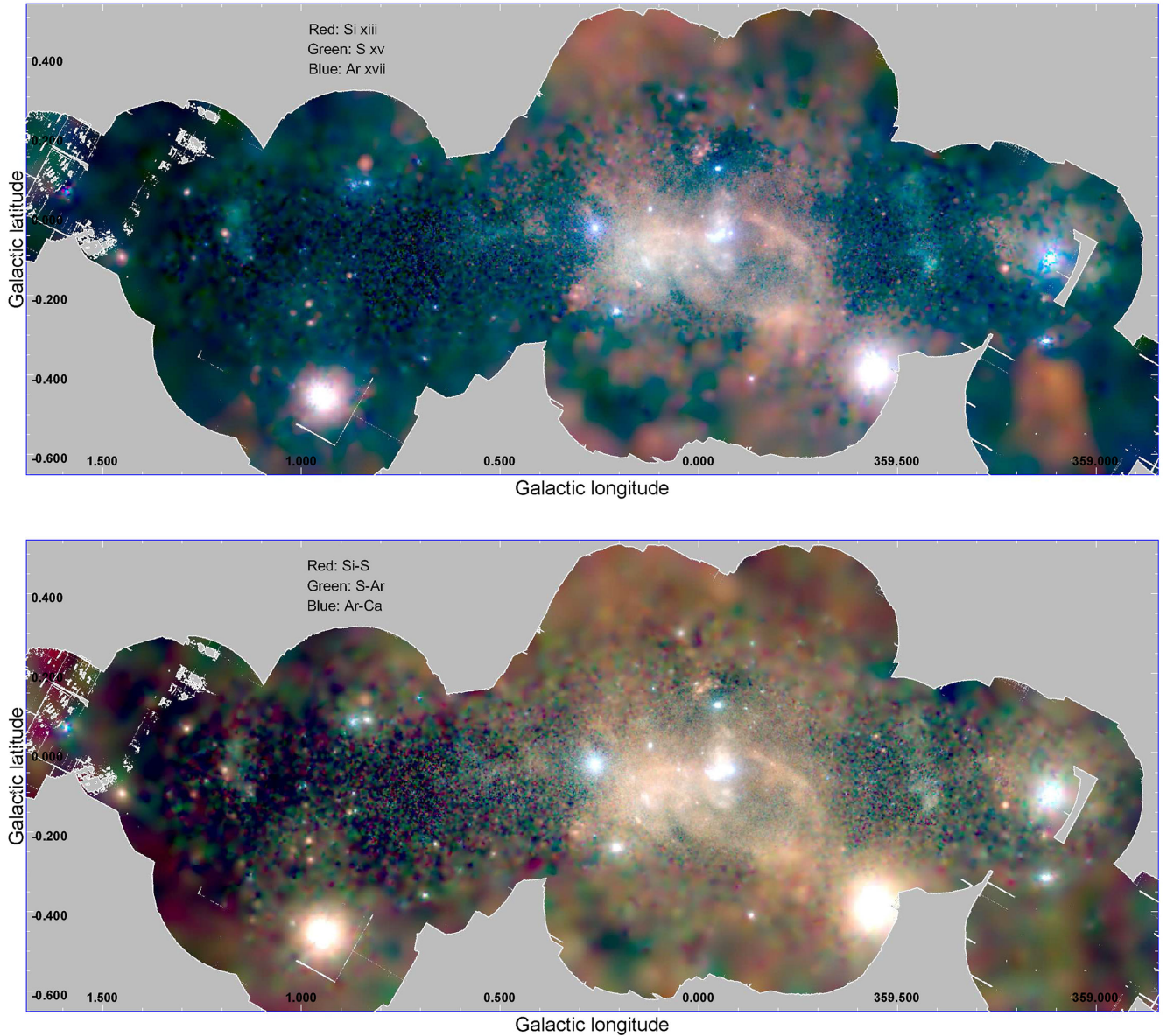
Figure 10. Top panel: soft lines (continuum unsubtracted) RGB image of the CMZ. The Si xiii line emission is shown in red, S xv in green and Ar xvii + Ca xix in blue. Bottom panel: RGB image of the energy bands between soft emission lines. The Si–S band emission is shown in red (see Table 1 for a definition of the energy bands), S–Ar in green and Ar–Ca + Blue–Ca in blue. The diffuse emission in this interline continuum is very similar to the soft emission line one, suggesting that the same process is producing both the lines and the majority of the soft X-ray continuum. The colour variations within the map are modulated primarily by abundance variations (top), temperature of the emitting plasma, continuum shape and absorption.
