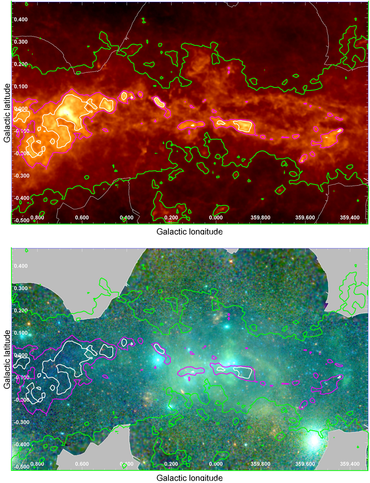
Figure 8. Top panel: neutral hydrogen column density distribution as derived from dust emission (Molinari et al. 2011). The image shows the N_H distribution in logarithmic scale from N_H = 4.5 \times 10^{22} up to 3.8 \times 10^{25} \text{ cm}^{-2} . The green, magenta and white contour levels correspond to N_H = 1.5 \times 10^{23} , 7 \times 10^{23} and 1.5 \times 10^{24} \text{ cm}^{-2} , respectively. Bottom panel: X-ray continuum RGB map (Fig. 3) with the column density contours overlaid.
