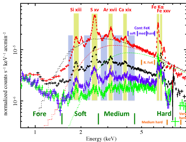
Figure 2. EPIC-pn spectra of the regions: G0.11–0.11 (red), Center Superbubble (black), G0.687–0.146 (green) and Sgr B1 soft (blue). In dark green are the energy bands of the broad GC continuum. In orange (bottom right) is shown the part of the hard energy band excluded in order to avoid contamination by Ni K \alpha , Cu K \alpha and ZnCu instrumental background emission lines. Yellow stripes show the energy bands of the soft and Fe K emission lines. Blue stripes indicate the regions selected for the determination of the amount of continuum underlying the soft lines. The dotted lines, from top to bottom, show the predicted emission of a source with a power-law spectrum (with slope \Gamma = 1.6 ) if absorbed by a column density of N_H = 3, 5 and 9 \times 10^{22} \text{ cm}^{-2} , respectively. The blue and orange labels indicate the selected broad energy bands for the determination of the continuum underlying the Fe K line emission.
