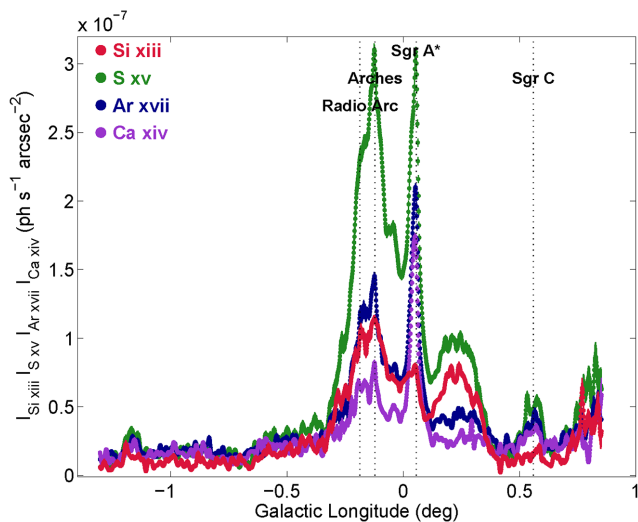
Figure 15. Longitudinal intensity profiles of the Si xiii (red), S xv (green), Ar xvii (blue) and Ca xiv (violet) emission lines, integrated over Galactic latitude within the magenta rectangular region shown in Fig. 14.
