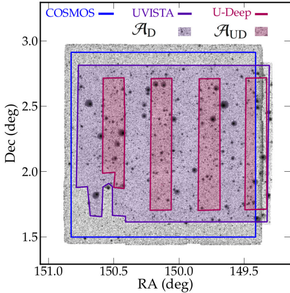
Fig. 1. Layout of the COSMOS field. The image in the background is the \chi^2 -stacked zYJHK_s image. The COSMOS 2 deg 2 field is enclosed by a blue line, while the UltraVISTA survey is inside the purple contour. UltraDeep stripes, where UltraVISTA exposure time is higher, are delimited by magenta lines. A purple (magenta) shaded area shows the Deep (UltraDeep) region used in this paper.
