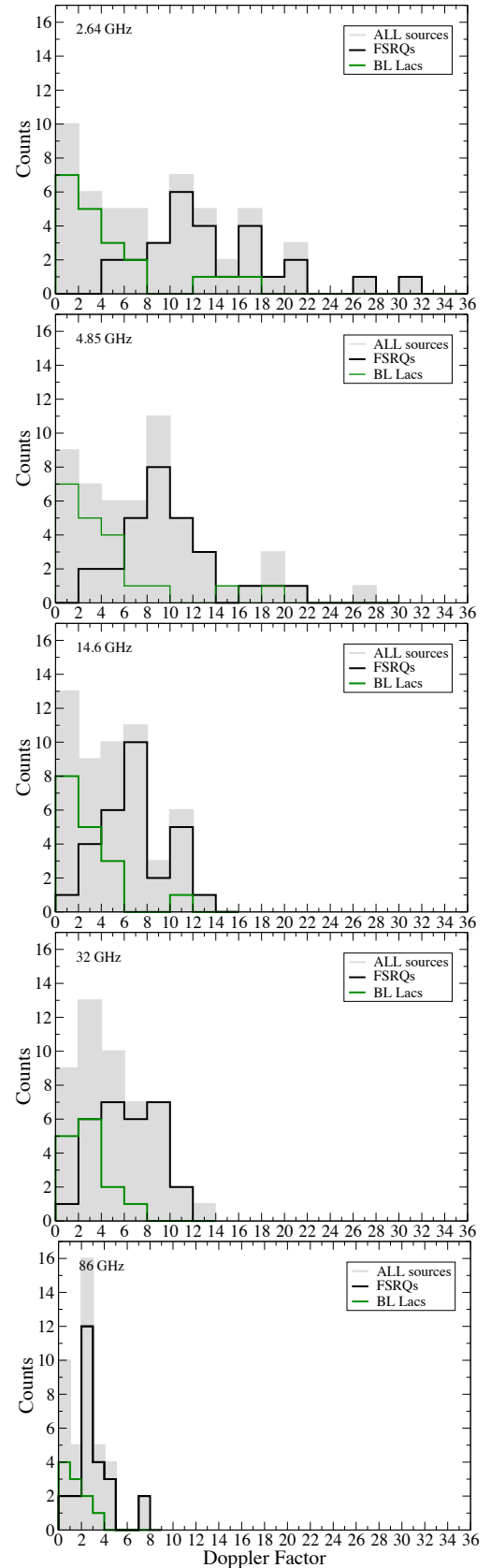
Fig. 5. Distributions of variability Doppler factors \delta_{var,eq} at selected frequencies: 2.64, 4.85, 14.6, 32 and 86 GHz from top to bottom, respectively. All sources (grey) are shown with FSRQs (black) and BL Lacs (green) superimposed. Note the systematic decrease of \delta_{var,eq} towards higher frequencies as well as the difference in the sample between FSRQs and BL Lacs (see text).
