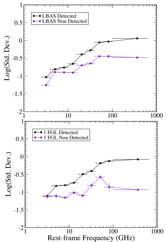
Fig. 8. The variability amplitude against rest-frame frequency for the Fermi LBAS detected/non-detected sources (upper panel) and 1FGL detected/non-detected sources (lower panel) of the F-GAMMA sample. y-axis: logarithmic average of the light curve standard deviations
