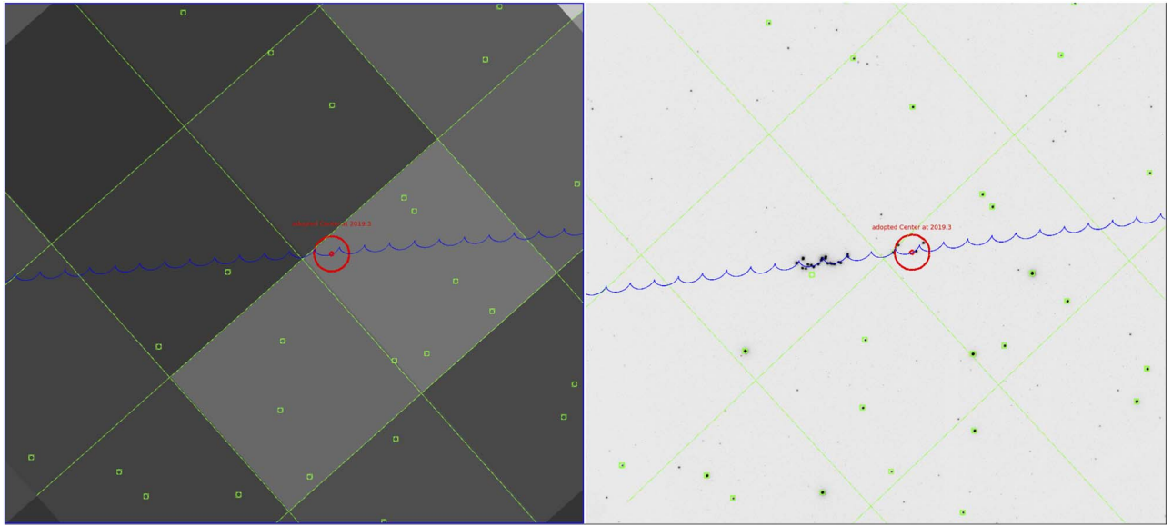
Figure 1. (Left) Finding chart of Luhman 16 AB on TESS image (tess2019107105933). Axes are aligned north up, east to the left, and the field of view (FOV) is about 66'' \times 60'' . (Right) Same FOV from the Hubble Space Telescope (HST) (from Bedin et al. 2017). Green lines indicate the pixel grid on the TESS images. The blue lines are the astrometric solution for the barycenter of the Luhman 16 AB system. The red circles highlight the adopted position for the barycenter at the epoch 2019.26 during which TESS observations were acquired, the smallest of which has a radius of 220 mas (indicative of the smallest separation between the two components). The green squares are the sources in the Gaia DR2 catalog.
