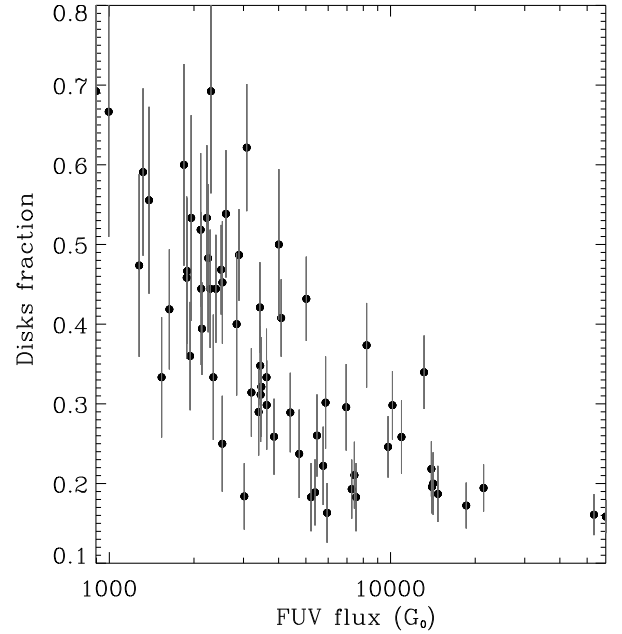
Figure 9. Left panel: maps showing the spatial variation of the disk fraction as in Figure 7. The overplotted contours mark the local FUV flux. The contour levels are 710.2, 2262.8, 3536.7, 6163.4, 11,087.3, 24,043.4 G_0 . Right panel: disk fraction vs. FUV flux in the bins of the same grid, showing only the values measured in bins with the relative error of the disk fraction smaller than 0.25.
