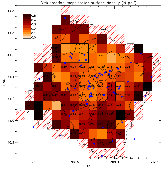
Figure 8. Left panel: maps showing the spatial variation of the disk fraction as in Figure 7. The overplotted contours mark the local stellar surface density. The contour levels are 0.7, 5, 17, 22, and 33 \text{N pc}^{-2} . Right panel: disk fraction vs. stellar surface density flux in the bins of the same grid, showing only the values measured in bins with the relative error of the disk fraction smaller than 0.25.
