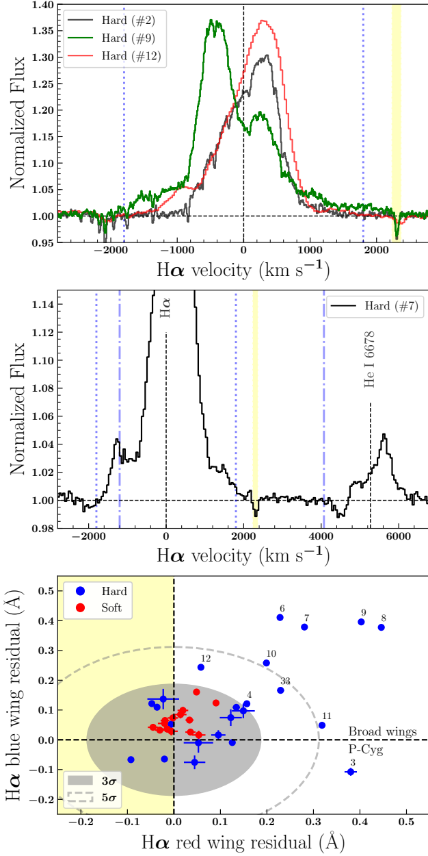
Figure 2. Evolution of H \alpha . Top panel shows the best examples for asymmetric lines (black, red) and broad emission line wings (green). Middle panel displays epoch #7, where P-Cyg profiles (He I-6678) and broad wings (H \alpha ) are detected. H \alpha also shows an absorption trough with a blue edge velocity of \sim -1200 km s ^{-1} . The two v_t inferred from P-Cyg profiles (He I-5876) at different stages of the outburst (dotted and dash-dotted lines at \pm 1800 and -1200 km s ^{-1} ) align very closely with the velocities of the H \alpha wind features. The dash-dotted line on the right corresponds to -1200 km s ^{-1} with respect to He I-6678. Yellow shading indicates regions contaminated by interstellar absorption. Bottom panel : H \alpha wings diagram. Epochs (note associated numbers) beyond the 5\sigma contour (dashed line) show conspicuous emission line wings. None of the soft-state data points (red dots) is located beyond the 3\sigma gray-shadowed area. The left regions of the diagram are forbidden for typical wind features (yellow shading).
