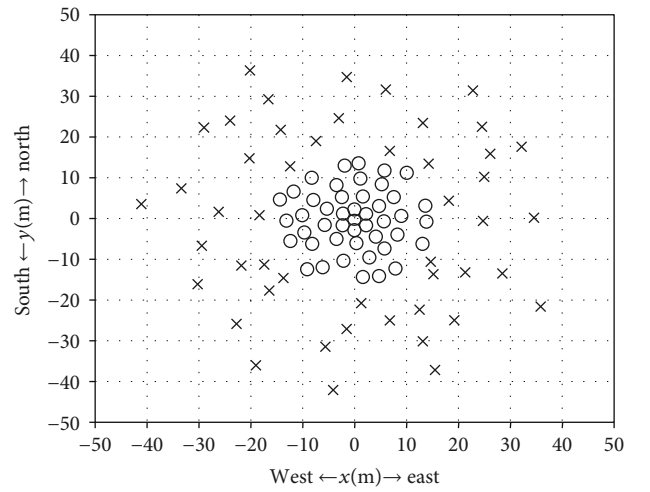
FIGURE 2: LBA geometry: the inner antenna distribution is the LBA-inner array (circles) and the outermost distribution is the LBA-outer array (crosses).
