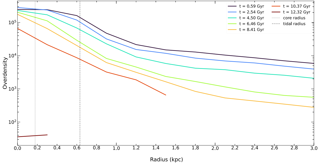
Figure 6. Radial distribution of overdensity for the fiducial simulation of Leo II ( \eta 60vCalc ).
