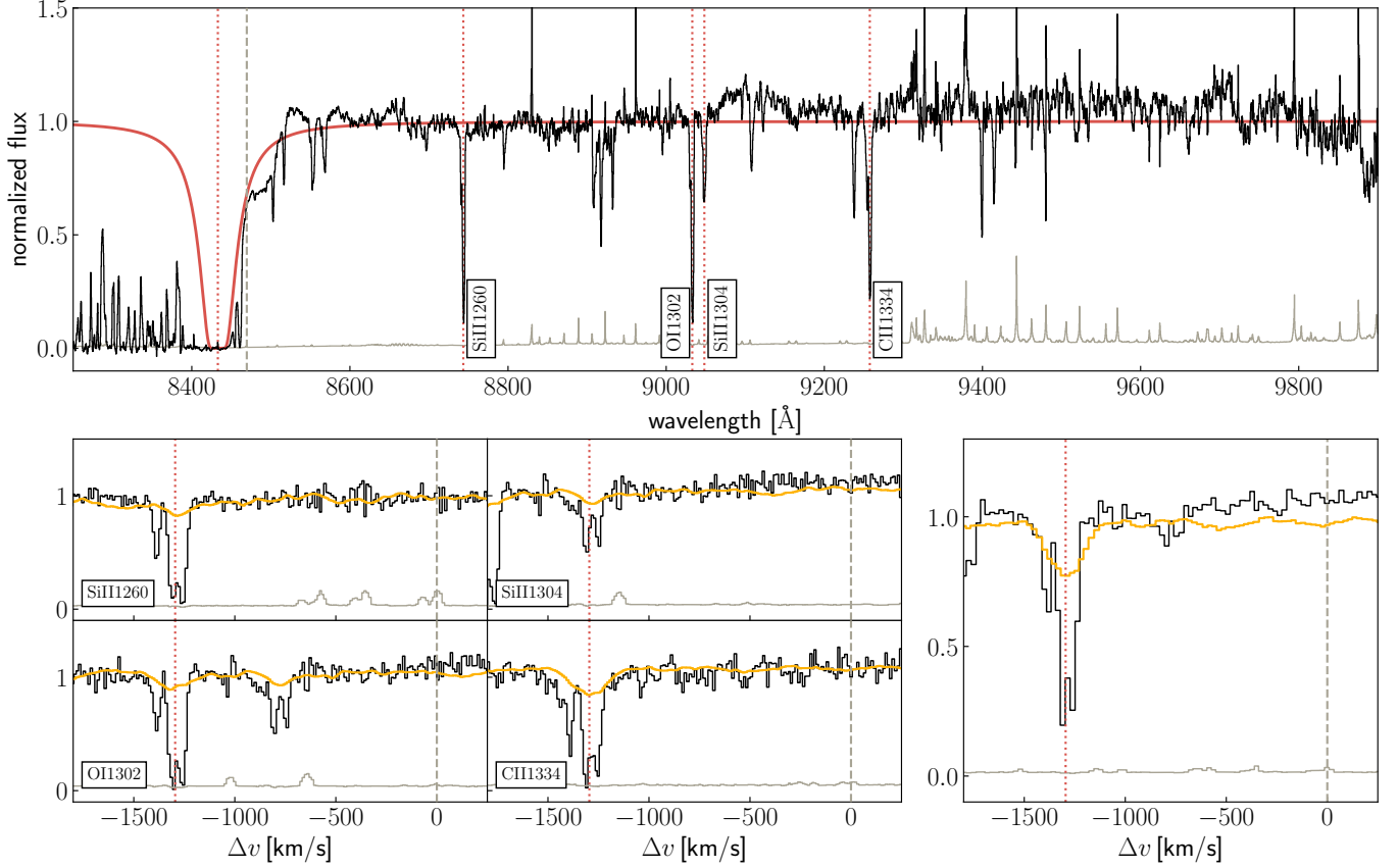
Figure 5. Optical quasar spectrum (black) showing a proximate absorption systems (red) in the vicinity of PSO J056-16 ( top ). The parameters of the absorption system, i.e. \log N_{\text{HI}} = 20.4 \text{ cm}^{-2} and b = 25 \text{ km s}^{-1} , are only fitted by eye. The spectrum at the locations of the low-ionization metal lines ( bottom left ) and the stack thereof ( bottom right ) show clear evidence for the presence an optically thick, self-shielding system. The yellow line represent a composite spectrum of 20 LLs (Fumagalli et al. 2011).
