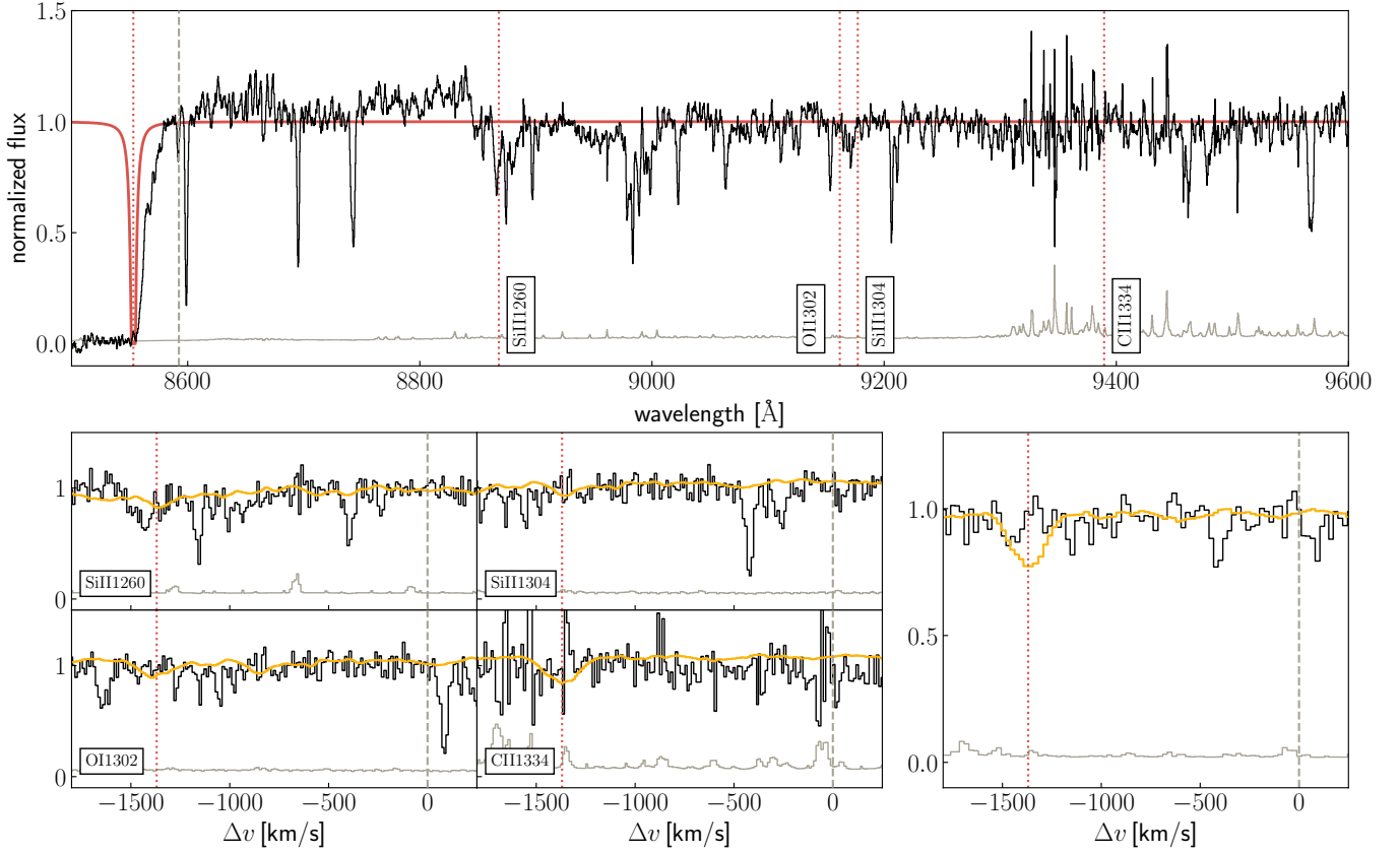
Figure 16. Same as Fig. 6 but for PSO J158–14.
