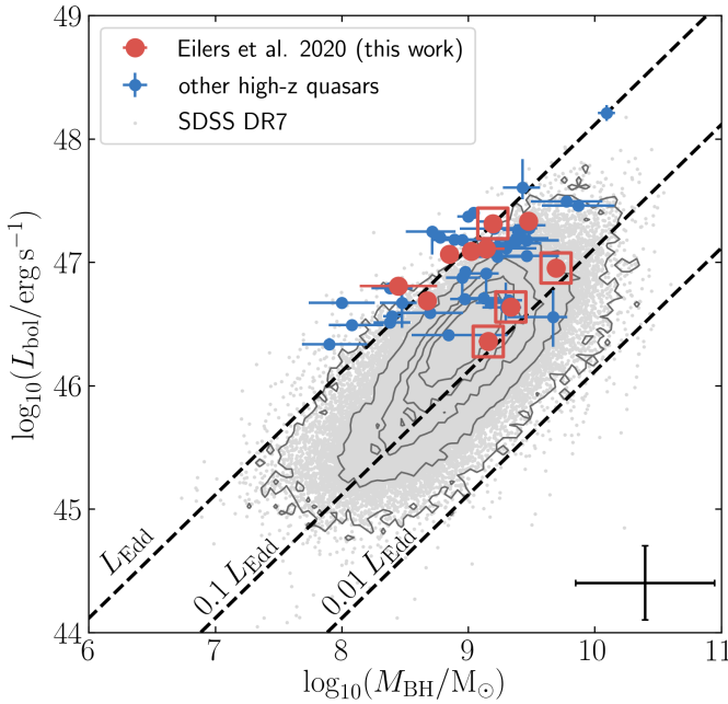
Figure 8. Relation between L_{\text{bol}} and M_{\text{BH}} for our new measurements (red) compared to a quasar sample at 0.4 \lesssim z \lesssim 2.2 from SDSS DR7 (grey), as well as several other z \gtrsim 5.8 quasars (blue). The red boxes indicate quasars with short lifetimes. The black dashed curves show regions with constant Eddington luminosity. The errorbar on the lower right corner indicates the size of the systematic uncertainties of approximately 0.3 dex and 0.55 dex on L_{\text{bol}} and M_{\text{BH}} , respectively.
