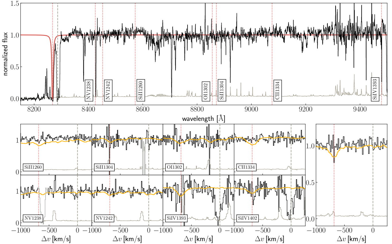
Figure 14. Same as Fig. 6 but for PSO J004+17. For this object we also show the locations of the high-ionization absorption, since these show evidence for an absorption system at the systemic redshift of the quasar (grey dashed lines). Wavelength regions (shown in light grey) around very prominent skylines, as well as around low-redshift absorption systems have been masked to avoid biases in the stack.
