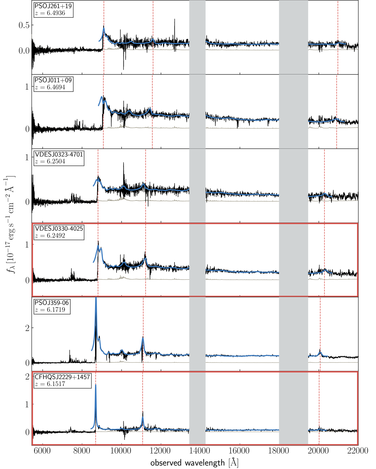
Figure 11. Same as Fig. 2 with quasar continuum estimates, shown in blue.
