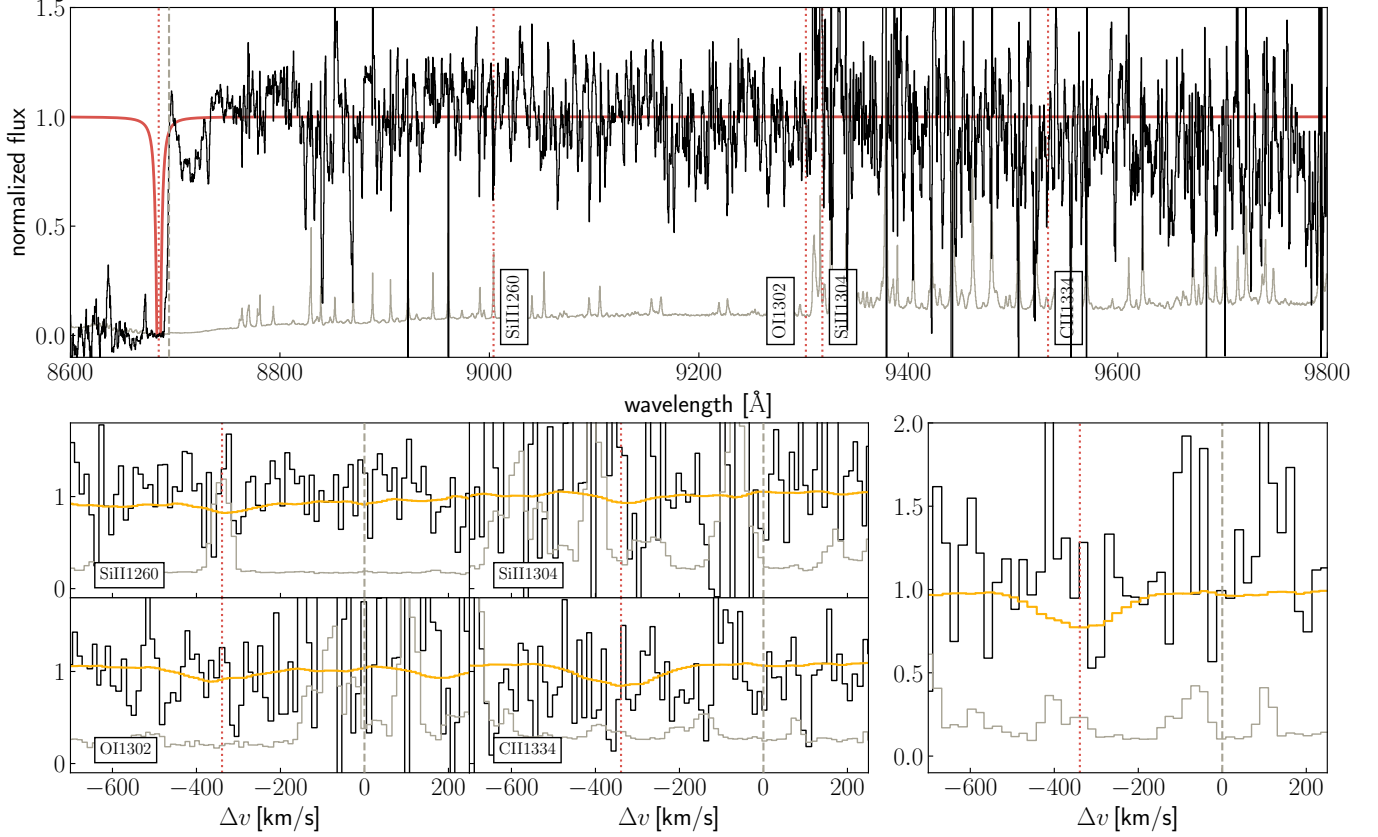
Figure 17. Same as Fig. 6 but for CFHQS J2229+1457.
