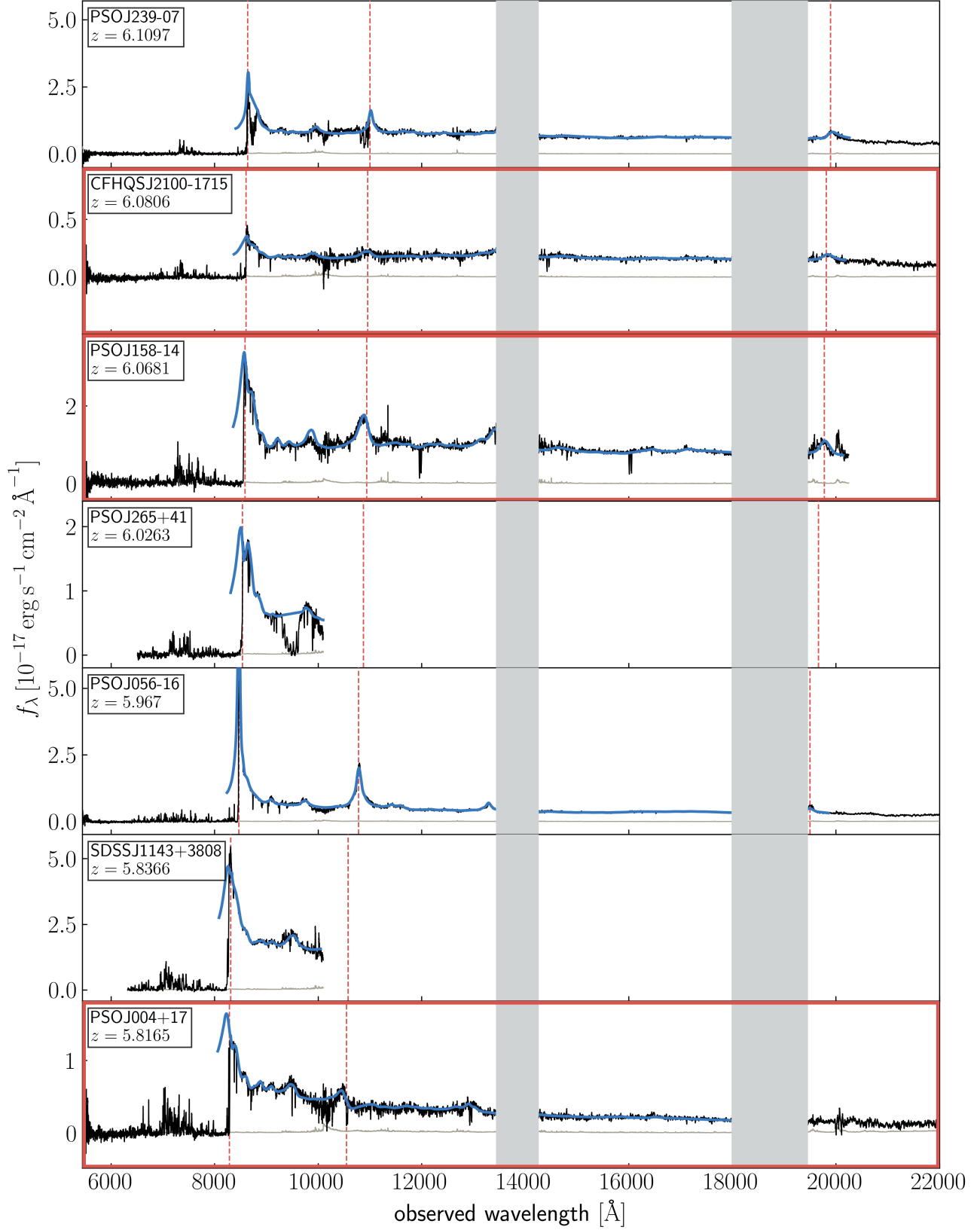
Figure 12. Same as Fig. 3 with quasar continuum estimates, shown in blue.
