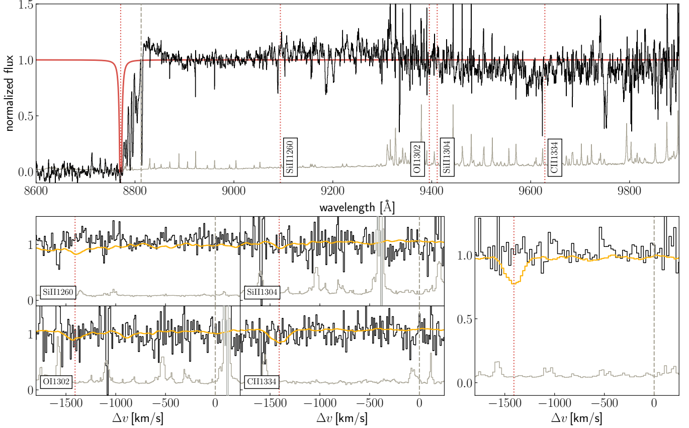
Figure 15. Same as Fig. 6 but for VDES J0330–4025. Wavelength regions around very prominent skylines (shown in light grey) have been masked to avoid biases in the stack.
