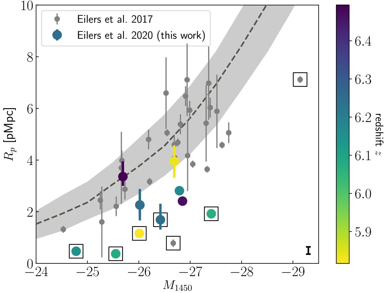
Figure 7. Proximity zone sizes R_p as a function of the quasars’ absolute magnitude M_{1450} . Our new measurements are shown as colored data points, whereas the grey square data points shows previous work (Eilers et al. 2017a). The grey dashed line and shaded region represents the median and 68th percentile of the distribution of 400 simulated proximity zones from radiative transfer simulations at z = 6 and \log t_Q = 7.5 yr (see Davies et al. 2016; Eilers et al. 2017a, for details), respectively. The seven quasars with extremely small proximity zones are indicated by the black boxes. The black errorbar in the bottom right indicates the systematic uncertainty on the R_p measurements with sub-mm redshifts, assuming a systematic uncertainty on the sub-mm redshift estimates of \Delta v = 100 \text{ km s}^{-1} .
