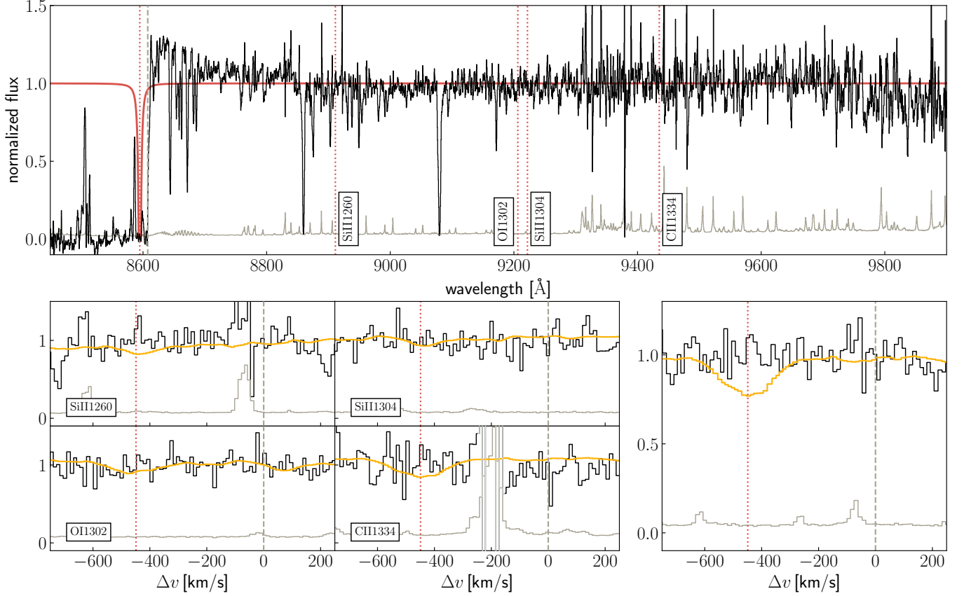
Figure 6. Optical quasar spectrum (black) showing a hypothetical absorption system (red) with parameters \log N_{\text{HI}} = 17 \text{ cm}^{-2} and b = 25 \text{ km s}^{-1} in the vicinity of CFHQS J2100–1715 ( top ). The spectrum at the locations of the low-ionization metal lines ( bottom left ) and the stack thereof ( bottom right ) do not show evidence for the presence of such a system. The yellow line represent a composite spectrum of 20 LLSs (Fumagalli et al. 2011). Wavelength regions around very prominent skylines (shown in light grey) have been masked to avoid biases in the stack.
