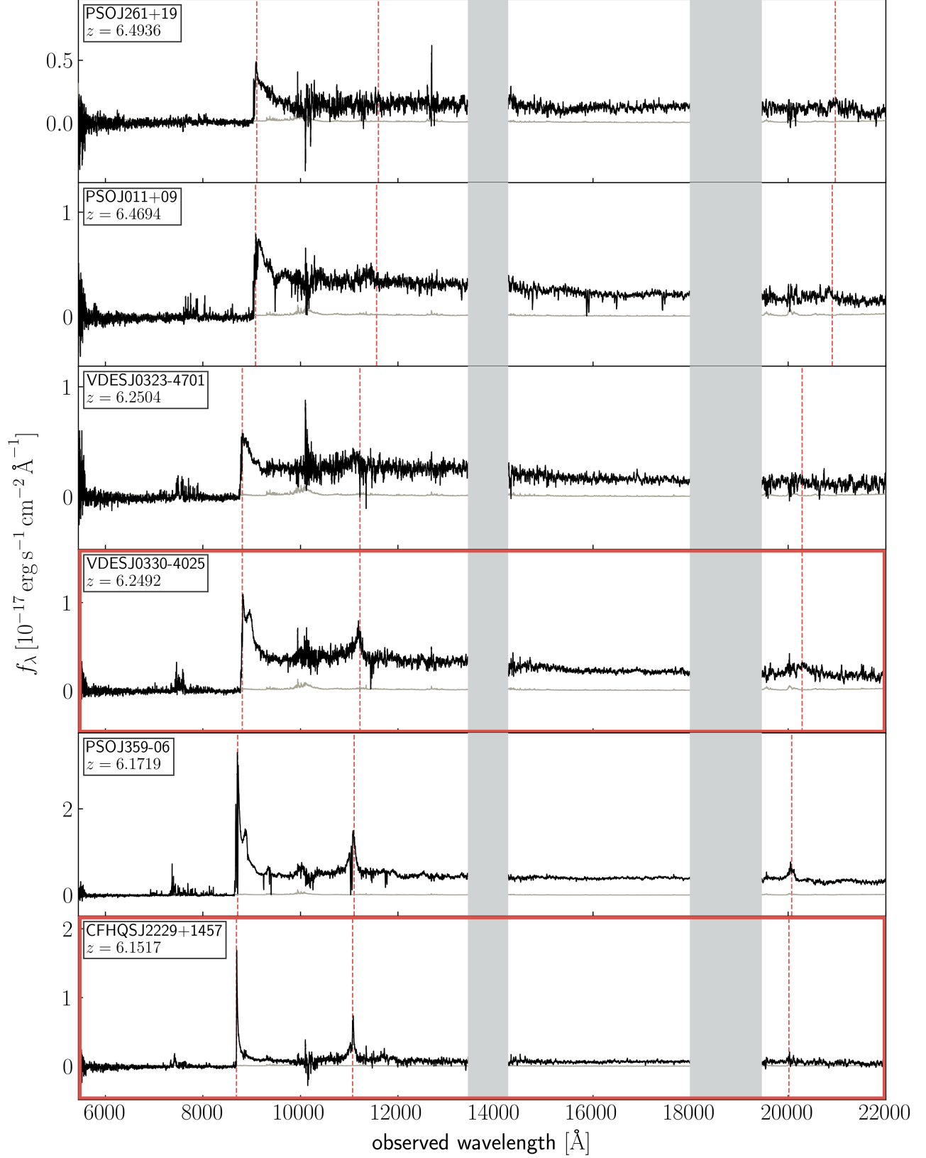
Figure 2. Spectra of the quasars in our sample. All spectra (black) are observed with VLT/X-Shooter, besides the spectra of the two quasars PSO J265+41 and SDSS J1143+3808, which have been observed with Keck/DEIMOS. Regions of large telluric absorption have been masked with grey shaded regions. The dashed red lines indicate the location of various emission lines, i.e. Ly \alpha at 1215.7 Å in the rest-frame, the C IV doublet at 1548 Å and 1550 Å, as well as the Mg II emission line at 2798.7 Å. All spectra and noise vectors (grey) have been inverse-variance smoothed with a 20 pixel filter. The red frames indicate quasars that exhibit very small proximity zones, i.e. R_{p, \text{corr}} \lesssim 2 pMpc.
