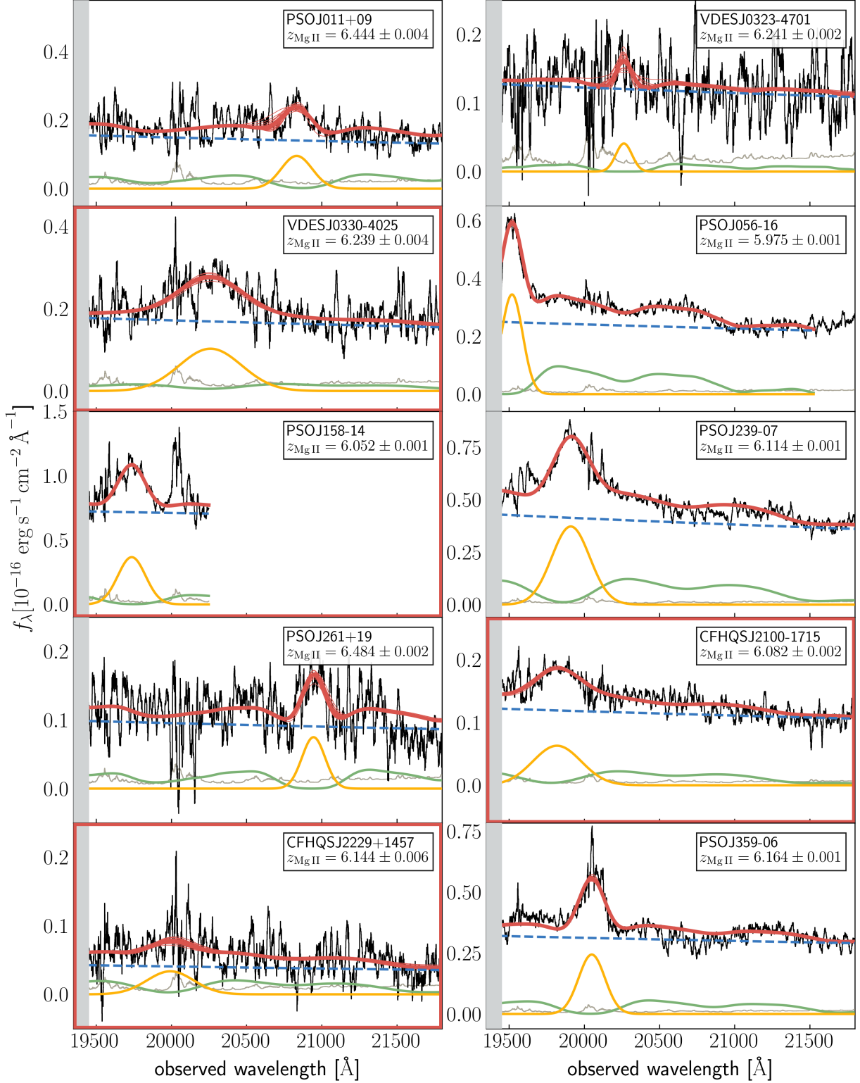
Figure 10. Best fits to the Mg II emission lines. We show all quasars in our sample that have NIR spectral coverage and their Mg II line does not fall into a region of high telluric absorption. The spectra around Mg II at \lambda_{\text{rest}} = 2798 Å and the corresponding noise vector have been inverse-variance smoothed with a 20 pixel filter and are shown in black and grey, respectively. The fit to the quasar emission (red curve), as well as its individual components are shown as the colored curves, i.e. a power-law continuum (blue dashed), the smoothed iron template (green), and a Gaussian for the Mg II emission line. Regions with large telluric absorption have been masked by the grey regions. The faint red lines show draws from the posterior distribution. The red frames show quasars that exhibit very small proximity zones and short lifetimes.
