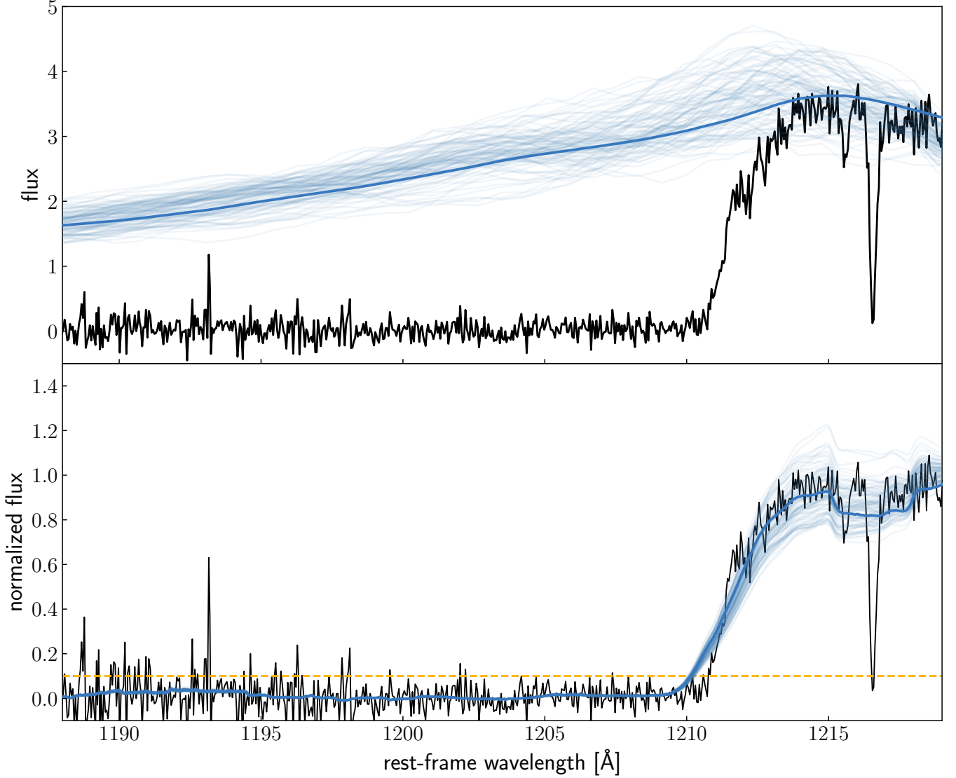
Figure 13. Example for analyzing the effects of the quasar continuum uncertainties on the proximity zone measurements. Top: Spectrum of PSO 158-14 (black) with 100 draws from the quasar continuum estimate including Gaussian noise (blue). Bottom: Continuum normalized quasar spectrum and the smoothed flux from the different draws of the continuum estimate, showing that the influence of continuum uncertainties is very small on the location of R_p , where the smoothed flux drops below the 10%-level (yellow).
