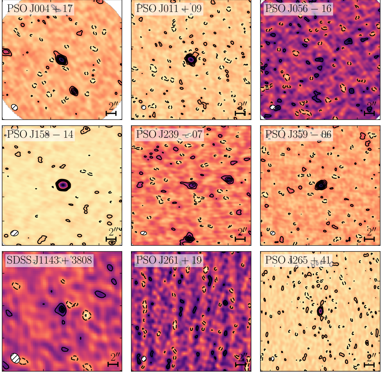
Figure 9. Dust continuum maps. The six quasars in the top and middle row show ALMA observations, whereas the bottom row shows our NOEMA data. Each panel is 25'' \times 25'' in size. Solid and dashed lines show the \pm 2, 4, 6, 8, 10\sigma isophotes.
