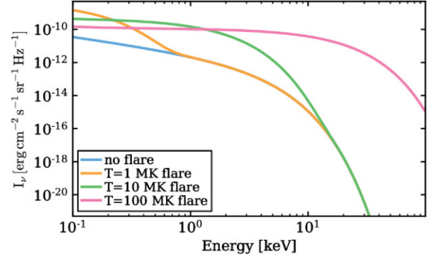
Figure 6. Specific intensity, I_v = \epsilon_v L , produced by 1, 10, and 100 MK flares (orange, green, and magenta curves, respectively). These spectra are used as an input in PRODIMO to derive a new disc solution. The blue curve shows the case without flare.
