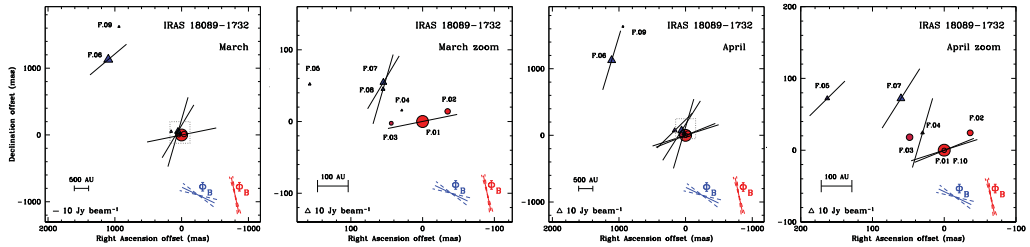
Figure 1. Masers identified in March (left) and April (right). The zoom is made on the region marked by the dashed grey boxes. Triangles and circles represent masers of the blue and of red group respectively. The different sizes of the triangles and the circles represent the intensity. Line segments mark the direction of the polarisation angle for the maser features that show linear polarisation. The average direction of the resulting magnetic field \Phi_B obtained for two groups of masers is indicated in the bottom right corners of each panel.
