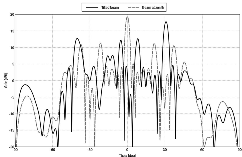
Figure 16. Array patterns for a station of SAD in the H plane with two different sets of phase coefficients for zenith and tilted pointing.
