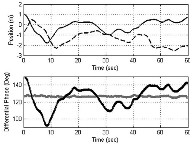
Figure 11. (top) Position of the UAV measured with the differential GNSS system: x coordinate (dashed) and y coordinate (continuous). (bottom) Measured differential phase shift for baseline V003-V007 (black) and residual phase after correction (gray).
