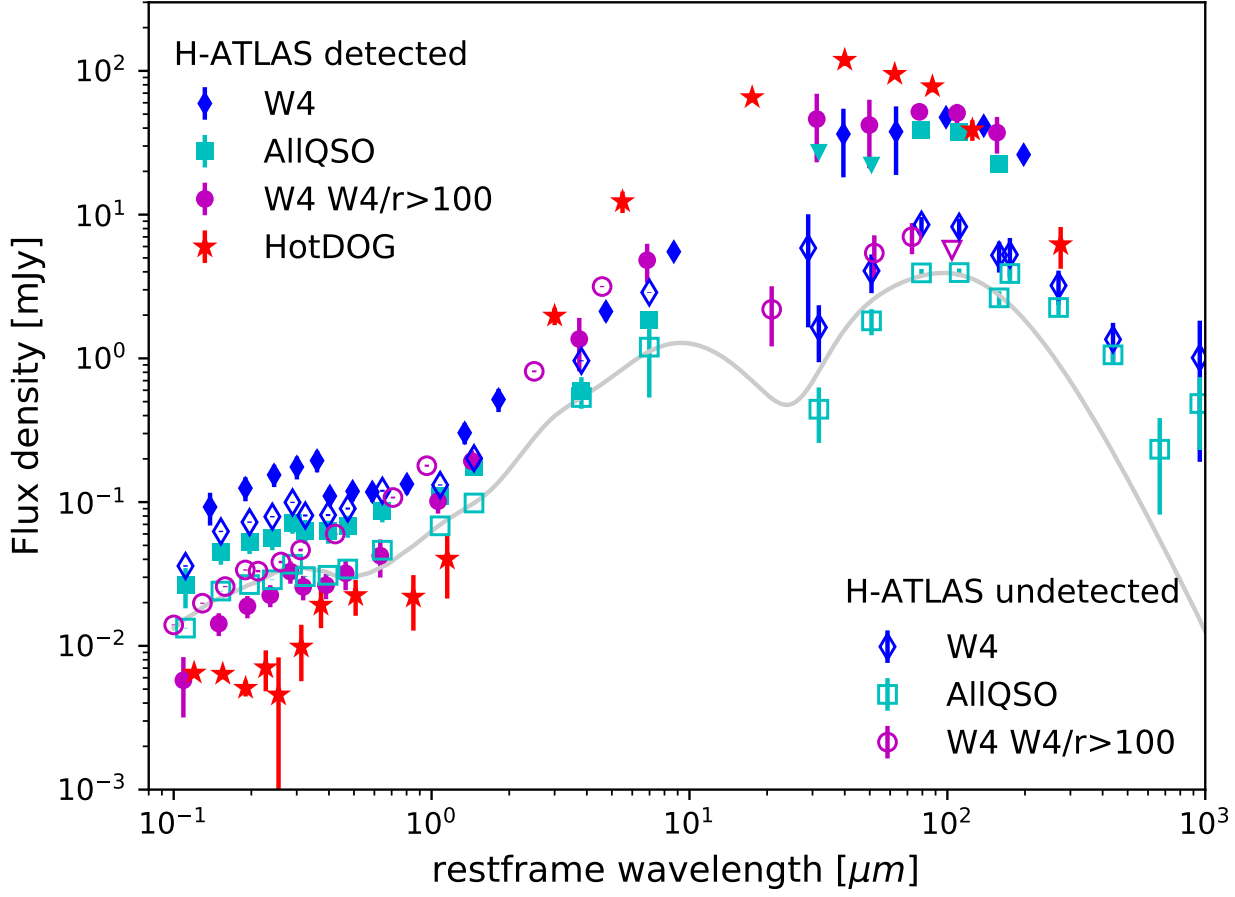
Figure 5. Averaged SEDs obtained for the different samples of QSOs in the redshift range 2.15 < z < 2.5 (or 1 < z < 5 for the H-ATLAS detected cases, see text for more details). Filled symbols correspond to SEDs where only sources detected in H-ATLAS catalogs are considered (no map-based stacking was needed in this case). On the contrary, the SEDs estimated considering also undetected H-ATLAS sources (stacking applied) are represented with empty symbols. Lower triangles indicate upper limits.
