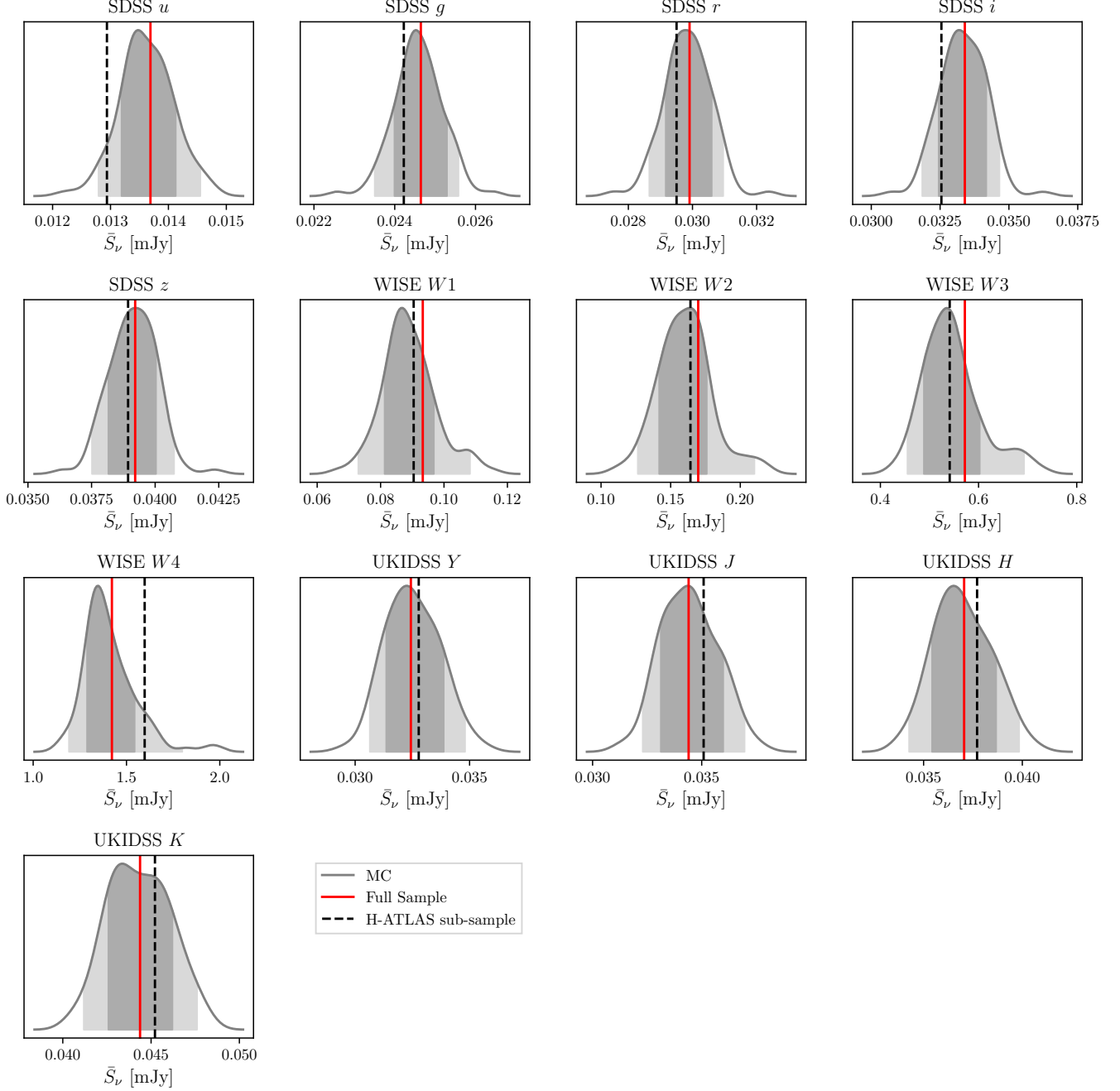
Figure 8. Assessment of the H-ATLAS sub-sample representativity. In each panel, the grey line shows a kernel density estimate of the distribution of the mean fluxes in a certain photometric band estimated from a set of 100 random sub-samples. The darker and lighter shaded areas indicate the \pm 1\sigma and \pm 2\sigma of the average flux distribution, evaluated as the (13.6, 86.4) and (2.1, 97.9) percentiles of the distribution respectively. The solid red and dashed black lines denote the average flux measured for whole QSO sample and the H-ATLAS sub-sample respectively.
