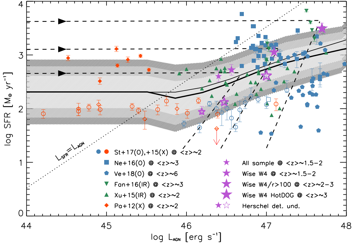
Figure 7. SFR vs. L_{\text{AGN}} plane between bolometric AGN luminosity and star formation rate in the host galaxy at z \gtrsim 2 . Dashed lines illustrate three typical evolutionary tracks (forward time direction indicated by arrows) from the in-situ coevolution scenario by Lapi et al. (2014, 2017) (see also Mancuso et al. (2016, 2017)) corresponding to \text{SFR} \sim 400, 1200, \text{ and } 4000 M_{\odot} \text{ yr}^{-1} . Dotted line represents the locus where the bolometric luminosity from AGN emission and from star formation are equal; galaxies to the right of such a line are prone to be affected by substantial AGN activity (see text). The thick solid line shows the average relationship and the shaded areas render its 1\sigma (light grey), 2\sigma (grey), and 3\sigma (dark grey) variance, computed as in Mancuso et al. (2016) taking into account number density of galaxies and AGNs, the relative time spent by individual objects in different portions of the tracks, and a far-IR detection threshold around \text{SFR} \sim 100 M_{\odot} \text{ yr}^{-1} . Literature data are from Stanley et al. (2015, 2017, circles), Netzer et al. (2016, squares), Venemans et al. (2018, pentagons), Fan et al. (2016, inverse triangles), Xu et al. (2015, triangles) and Page et al. (2012, diamonds). Red symbols refer to X-ray selected AGNs, blue to optically-selected AGNs, and green to mid-IR selected AGNs; the SFR measurements are obtained from far-IR observations with Herschel , both via detections (filled symbols) and via stacking (empty symbols); the sample by Venemans et al. (2018) is based on detections from ALMA millimetric data. Results from this work are illustrated as magenta stars for the overall sample at \langle z \rangle \sim 1.5-2 (tiny stars), for WISE W4-detected galaxies at \langle z \rangle \sim 1.5-2 (small stars), for WISE W4-detected galaxies with W4/ r -band luminosity ratio exceeding 100 at \langle z \rangle \sim 2-3 (medium-size stars), and for the unique HotDOG falling in the Herschel -ATLAS survey area at z \sim 3 (big stars); filled stars refer to far-IR detections with Herschel and empty symbols to stacked measurements (see Table 3 for more detailed information on photometric redshift). The thin solid black line is the average relationship obtained according to the AGN variability model (Hickox et al. 2014; Stanley et al. 2015, 2017, see text for details).
