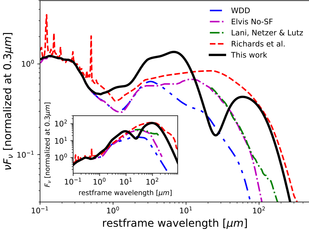
Figure 6. Comparison of the mean SED reconstructed in this work in the redshift range 2.15 < z < 2.5 (solid black line) with classic templates from literature. We show the SED from Richards et al. (2006) obtained using SDSS-selected QSOs in combination with Spitzer data (dashed red line), the template by Elvis et al. (1994) as revisited by Xu et al. (2015) from star formation in the host galaxy (dot-dashed magenta), and the WDD template by Lyu et al. (2017). Moreover, we have also plotted the most recent intrinsic AGN SED derived by Lani et al. (2017, green line).
