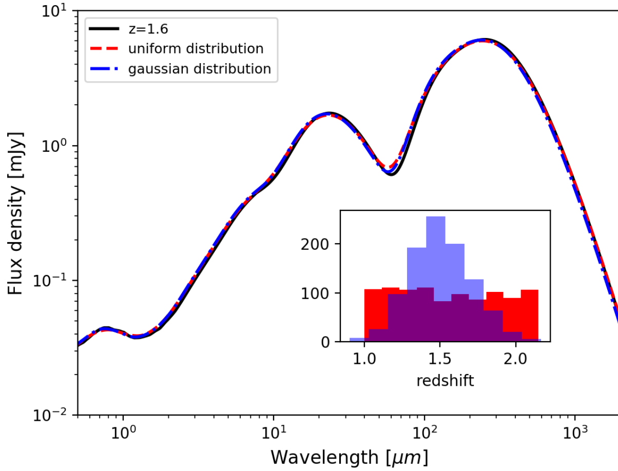
Figure 9. Results of the simple test using two different methodologies to estimate the average SED (see text for more details): main sample of QSOs in the first redshift bin ( 1.0 < z < 2.15 ) derived at the mean redshift ( z = 1.6 , black solid line ); rest-frame averaged SED considering an uniform ( dashed red line ) and a gaussian ( dot-dashed blue line ) redshift distributions inside the redshift bin.
