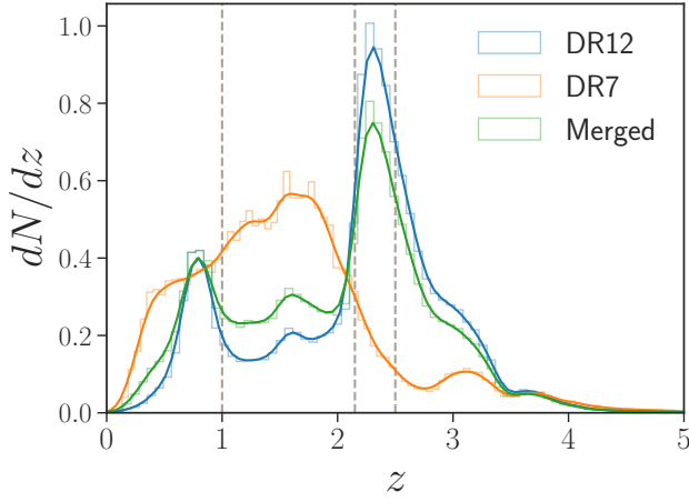
Figure 1. Unit-normalized redshift distribution of the individual SDSS DR7 (orange) and DR12 (blue) QSO catalogs, as well as the merged sample (green) used in this work (after the radio-loud cut has been applied). The vertical dashed lines represent the redshift bins employed in our analysis. The solid smooth lines represent kernel density estimates to the underlying redshift distributions.
