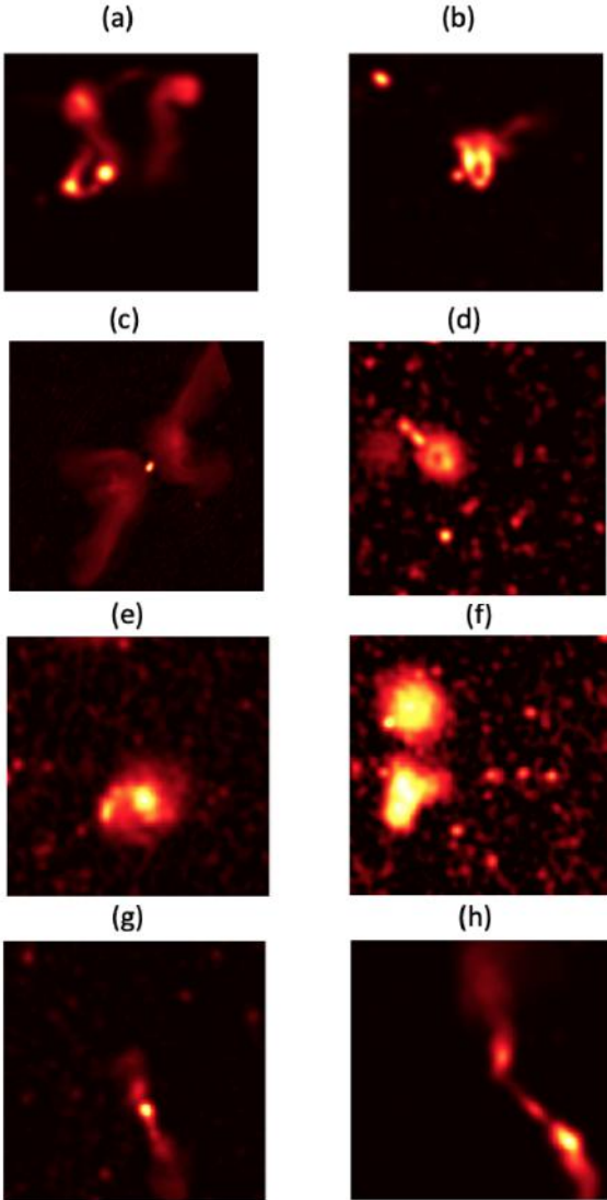
Figure 5. Examples of objects found within frames sampled above the 99th percentile complexity value from the EMU-PS Complexity Scan. These examples illustrate the breadth of objects found within frames in the complexity tail including, (a) the unusual source PKS 2130-538 (Otrupcek & Wright 1991) known as the Dancing Ghosts (Norris et al. 2021b), (b) a bright wide angle tail source on 2MASX J21291901-5053040 in cluster Abell 3771, (c) the large X-shaped radio source PKS 2014-55 (2MASX J20180125-5539312), (d) two odd radio circles, EMU PD J205842.8-573658 (ORC2) and EMU PD J205856.0-573655 (ORC3), (e) a face-on spiral galaxy NGC 7125, (f) 2MASX J20483764-4911157 FR-II remnant, (g) DES J202818.12-492408.4 FR-I potential Double-double radio galaxy and (h) FR-I extended radio source with host galaxy 2MASX J21512991-5520124.
