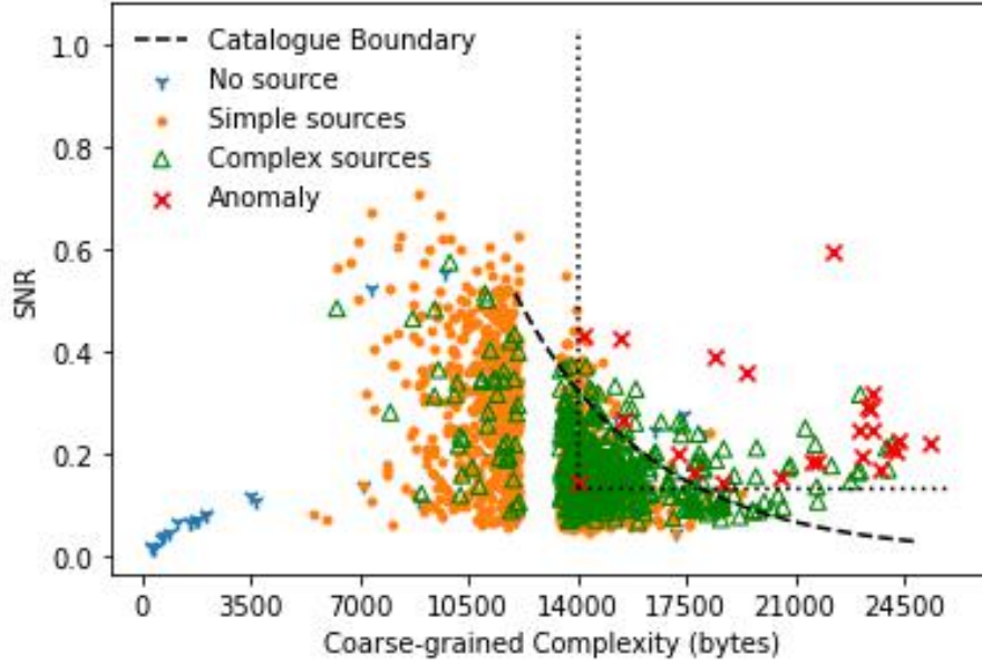
Figure 7. Scatter plot showing the coarse-grained complexity and the signal-to-noise ratio (SNR), and the relationship between them, for the EMU-PS zoo sub-sample inclusive of the enrichment sample (n=1627). The figure shows the classification of frames derived through consensus from the zoo (Anomaly in the EMU Zoo) and the function based catalogue boundary for anomalies (Catalogue Boundary) with its exponential form shown in this figure and expressed in terms of a log ratio adjustment of a lower bound complexity value in equation 4.
