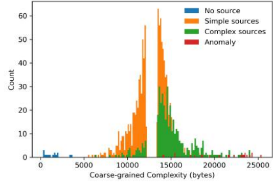
Figure A1. Histogram partitioned by consensus votes from the zoo. Bins in the range 12,200 bytes to 13,400 bytes were omitted as described in appendix A.
