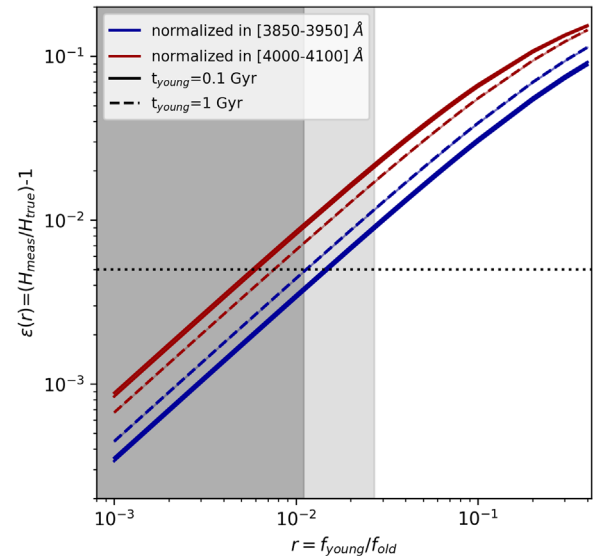
Figure 7. Impact on the measure of H(z) of a young component with fraction r with respect to the old component. The different colors show the effect when the spectra are normalized in different wavelength ranges ([4000–4100] Å for the red curves, [3850–3950] Å for the blue curves), while the different line styles represent different ages of the young component (0.1 and 1 Gyr). The gray shaded areas show the ranges of r allowed by the data in Moresco et al. (2012a, 2016b) averaged across all redshifts (darker at 1\sigma , lighter at 2\sigma ), and the black dotted line shows an error \epsilon(r) = 0.5\% . The shaded area (barely visible) between the curves represents the uncertainty due to different SPS models.
