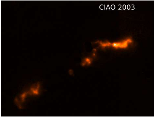
Fig. H.2. (Online movie) H_2 line structure variations between 2003 and 2020.
