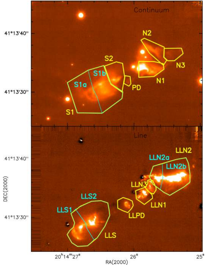
Fig. 2. Jet decomposition in polygons. Top panel: \text{Bry} -filter image of IRAS 20126+4104 obtained with LUCI1 and the AO system SOUL, overlaid with the polygons used for the photometry in the continuum. The adopted designation is labelled. We note that polygon S is composed of S1 and S2, and S1 is further subdivided into S1a and S1b. Bottom panel: pure H_2 line emission image of IRAS 20126+4104 obtained with LUCI1 and the AO system SOUL, overlaid with the polygons used for the jet photometry. The adopted designation is labelled. We note that polygon LLS is composed of LLS1 and LLS2, and LLN2 is subdivided into LLN2a and LLN2b.
