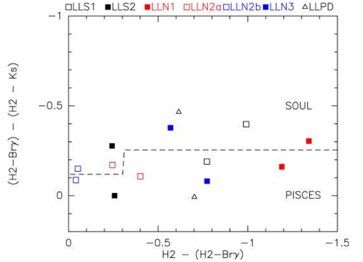
Fig. G.1. Difference (in magnitudes) between the pure line flux in the polygons after continuum correction from the Bry image, ( H_2 - \text{Bry} ) and the K_s image, ( H_2 - K_s ) vs the continuum contamination (in magnitudes) in the polygons estimated as the difference between the total flux measured in the H_2 band and the line flux corrected using the Bry image ( H_2 - \text{Bry} ). The symbols refer to the polygons in Fig. 2, as explained at the top of the box. Two datasets have been used (PISCES 2012 and SOUL 2020).
