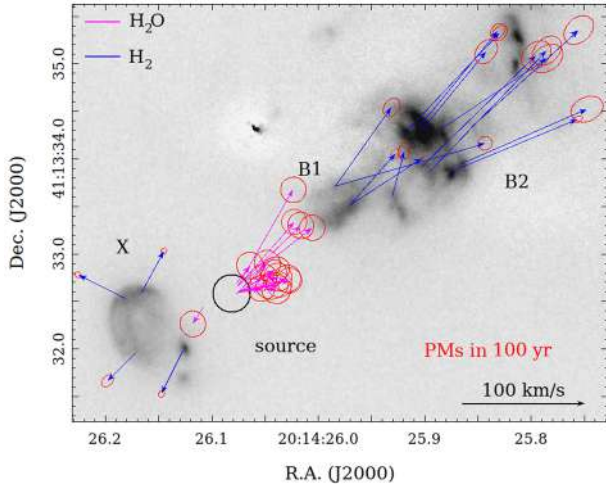
Fig. 15. Zoom-in on Fig. 8 around the source showing \text{H}_2\text{O} maser proper motions (magenta arrows) as measured by Moscadelli et al. (2011) and \text{H}_2 proper motions (blue arrows) from this paper. Red ellipses mark the uncertainties on PMs. The black circle shows the position of the protostellar continuum at 1.4 mm from Cesaroni et al. (2014).
