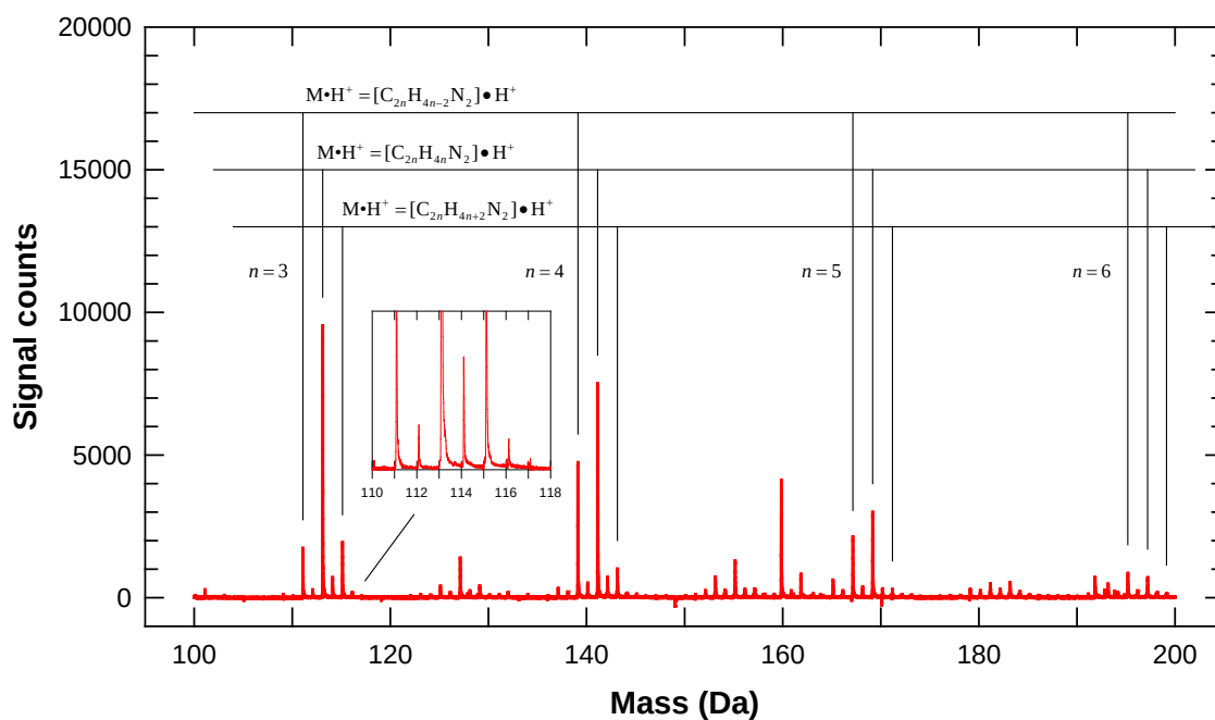
794 Fig. 5 DART high-resolution mass spectrum of the chromophore-containing deposit 795 produced in Experiment No. 1. Four groups of 3 main members, each 796 containing two N atoms, are shown and are interpreted as combinations 797 of aliphatic azine, azo, and diazo hydrocarbons. The inset shows details of 798 the mass peak profiles and presence of heavier C- and N-isotopes.
