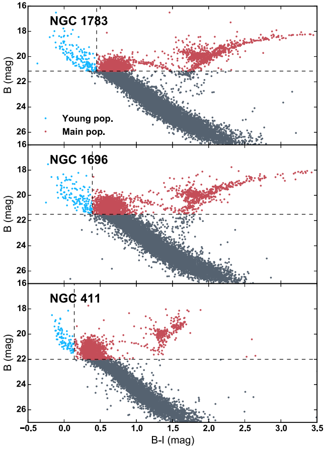
Figure 1. Selection of young (blue dots) and main ( \sim 1.5 Gyr old – red dots) populations from the CMDs (before decontamination) for the LFs (cf. Fig. 2) and radial profiles (cf. Fig. 8).
