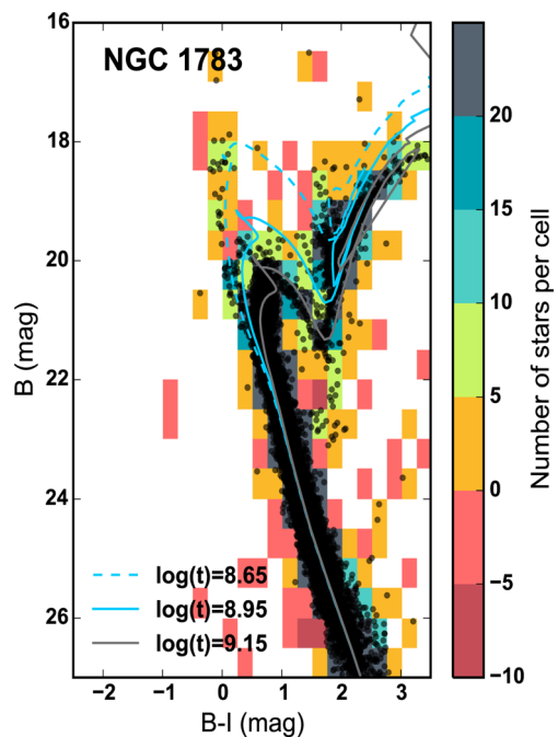
Figure 5. CMD of NGC 1783 produced by L16’s decontamination technique. In colour, we represent the number of star/cell. The negative values represent the grid cells where there were more stars in the reference field than in the cluster region.
