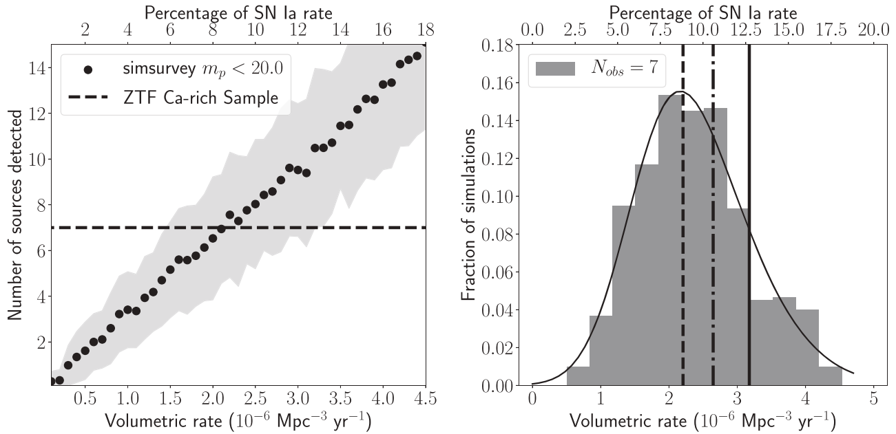
Figure 25. Estimate of the volumetric rate of Ca-rich gap transients with simulations of the ZTF survey using the simsurvey code. (Left panel) We show the number of sources passing our selection criteria for the CLU experiment as a function of the input volumetric rate (see text). The points and error bars are the mean and standard deviation of the number of transients recovered as a function of the volumetric rate, while the dashed black line shows the observed number of sources in the experiment. (Right panel) The fraction of simulations producing the observed number of transients as a function of the input volumetric rate. The dependence is fit with a skewed Gaussian distribution shown by the solid line, which we use to derive the best estimate of the volumetric rate and its confidence interval (see text). The dashed line shows the mean of the distribution, the dotted-dashed line shows the rate after correcting for galaxy catalog incompleteness, and the solid line shows the rate estimate after accounting for the transients missed beyond 100'' from their host galaxies.
