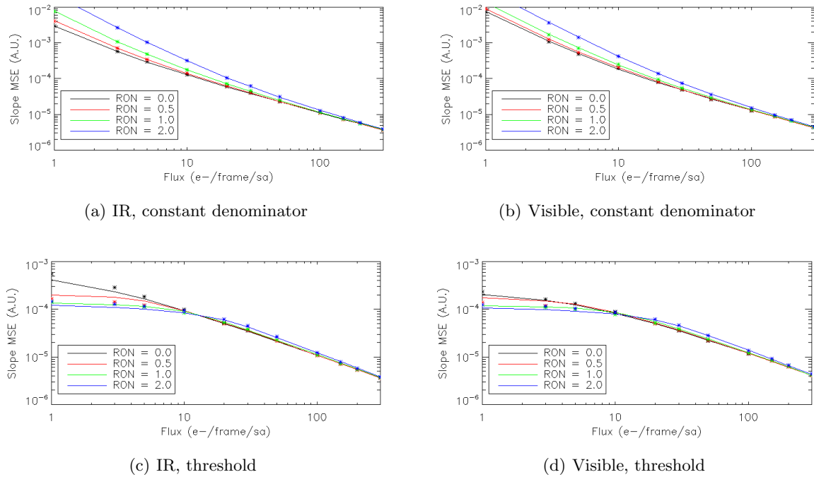
Figure 1. Slope error variance as a function of flux for different values of RON, with a constant denominator (top) or a threshold at 0 (bottom). The pupil sampling is 2 \times 2 and the FoV size is 50 pixels. Top and bottom left: diffraction-limited (spot FWHM = 17 mas) IR sensor with 10 mas pixels, FWHM of WCoG = 2 pixels, background + dark = 0.2 e-/pixel. Top and bottom right: seeing-limited (spot FWHM = 0.2") visible sensor with 100 mas pixels, FWHM of WCoG = 2 pixels, background + dark = 0.53 e-/pixel. Solid lines: theory. Symbols: simulations.
