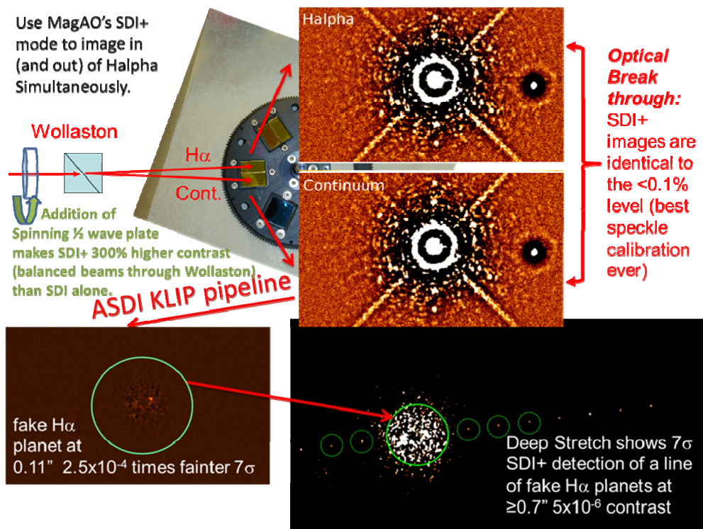
Fig 12: examples of fake planet sensitivity with SDI+
