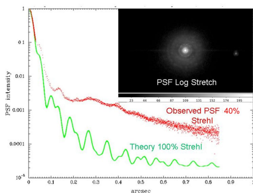
Fig 5: Deep PSF (40% Strehl) at 0.98\mu\text{m} PSF (140 nm rms WFE with just 200 modes). Modified from Close et al. 2013. Note how the 35 mas resolution of the PSF allows for a raw contrast of 500 at just 0.1'' separation. In this manner good inner working angles and contrasts can be achieved with visible AO even if the Strehls are lower than in the NIR.
