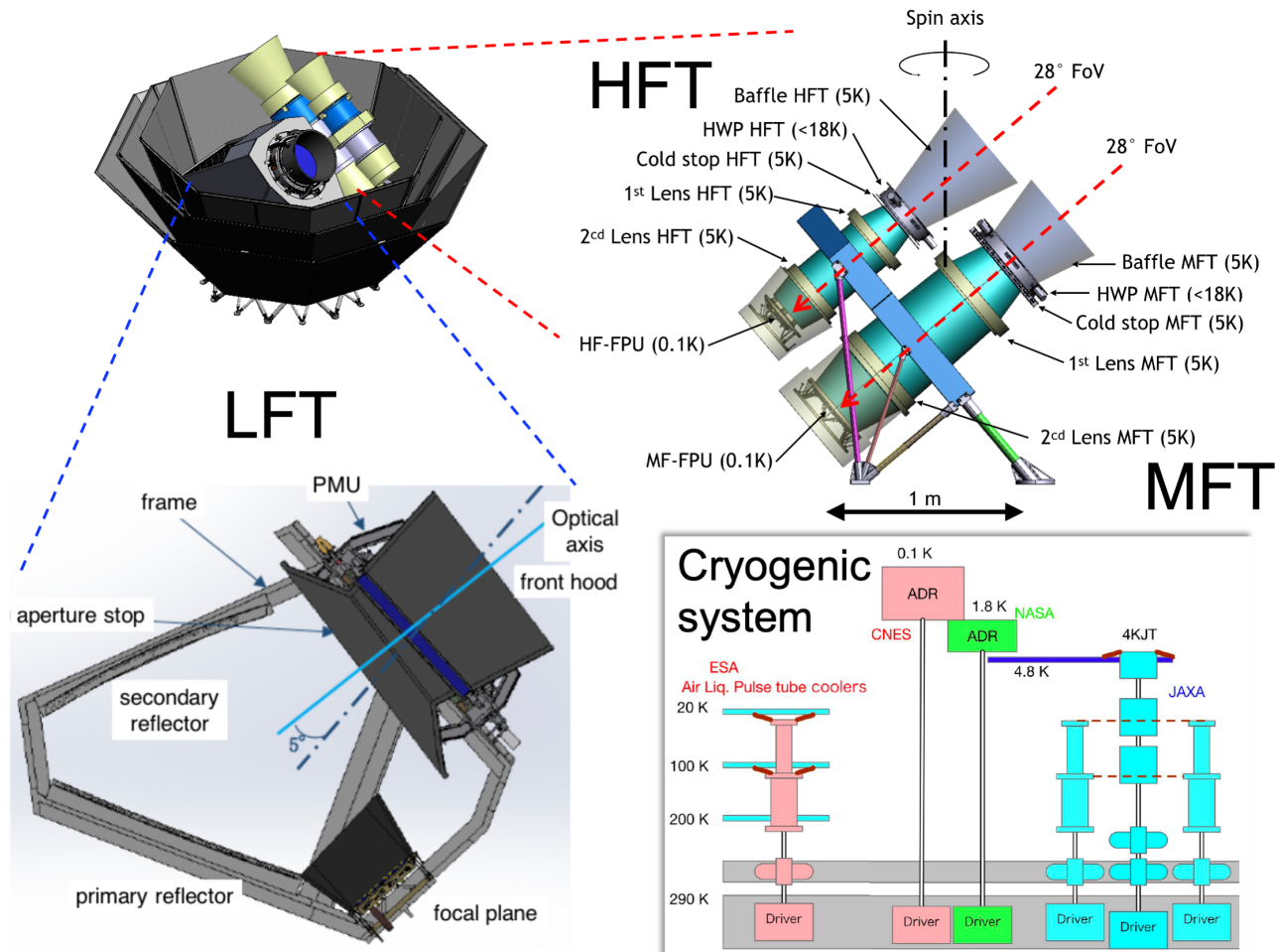
Figure 4. Overview of the payload module (PLM).
