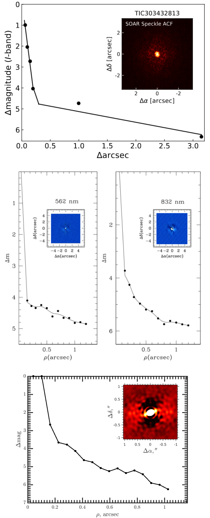
Fig. 2. High-angular-resolution imaging observations of the target. Top: speckle imaging obtained at 4.1-m Southern Astrophysical Research (SOAR) telescope. Middle: speckle imaging obtained at 3.5-m Wisconsin-Indiana-Yale-NOIRLab (WIYN) telescope. Bottom: speckle imaging obtained at 2.5-m telescope at the Caucasian Observatory of the Sternberg Astronomical Institute (SAI).
