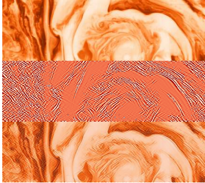
Figure 11. Waves over the cyclone #2 at the North Pole. Upper panel: original JIRAM image; central panel: result of the 2D Fourier high-pass filtering on the original image; lower panel: superimposition of the central panel to the upper panel.
