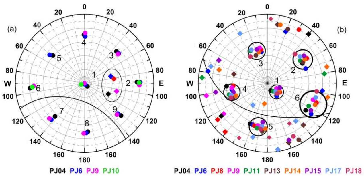
209 210 Figure 4. Position of the cyclone centers (dots) during the observation period for North pole [panel 211 (a)] and South pole [panel (b)]. The colors identify the different perijoves. The black circles indicate 212 the variation of the position of the southern cyclone centers and are centered at the average position 213 measured in the all period of observations. The diamonds represent the position of the different 214 anticyclones with diameters larger than 1000 km. The oval in panel (a) identify the different 215 positions of the same anticyclone during the different reported perijoves. 216
