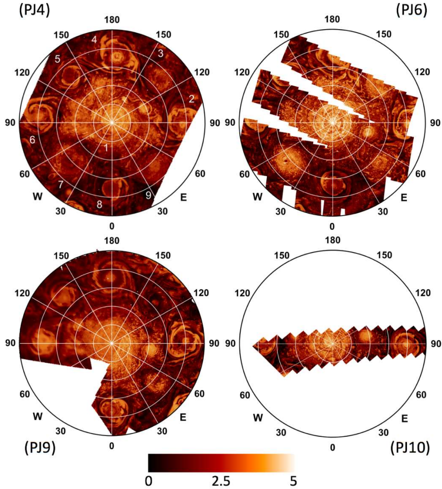
129 Figure 1. North pole during PJ4, PJ6, PJ9 and PJ10 (from top to bottom al left from right). Whitish 130 colors indicate higher optical depth ( \tau ), i.e. thicker clouds. Cyclone numbering: the polar cyclone is 131 #1; the cyclone at 90E is #2; the numbering proceeds counterclockwise from #3 to #9. The color bar 132 on the bottom indicates the value of \tau . 133 134 135
