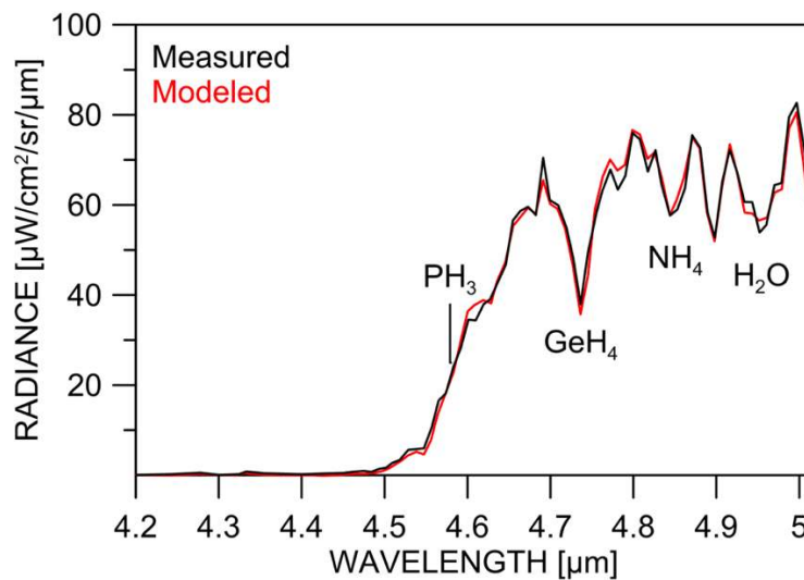
Figure 7. Comparison between a measured and a reconstructed spectrum between 4.2 and 5 \mu\text{m}
