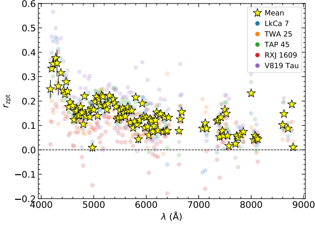
Figure 5. The zero-point of relative veiling as a function of wavelength. Yellow stars are the final r_{\text{zpt}} determined by averaging the individually measured r_{\text{zpt}} from different stellar templates in colored dots in the background. The shape resembles the relation between relative veiling and wavelength.
