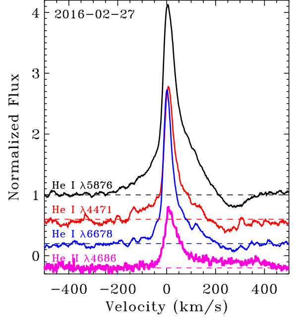
Figure 13. He I absorption, seen here to \sim 300 - 400 \text{ km s}^{-1} in three lines on 2016-02-27, an epoch with strong accretion. The He II \lambda 4686 line (bottom, pink) has emission that extends out to 450 \text{ km s}^{-1} .
