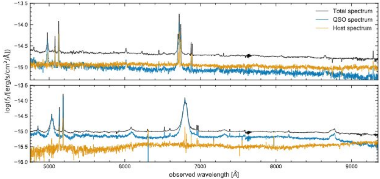
Fig. 6. Result of the iterative AGN-host deblending for HE 0108–4743 and HE 0351+0240 as two examples. 3''/2 aperture spectra centered on the QSO position are shown in both cases extracted from the original data (black line), the AGN contribution (blue line), the host galaxy contribution (orange line).
