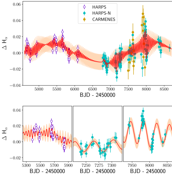
Fig. 5. Top: model obtained for the H\alpha time series using Gaussian Processes to treat the rotation signal and a sinusoidal function to treat the long-term signal. The shaded regions indicate the 1\sigma confidence band of the GP model. Bottom: zoom on different time windows.
