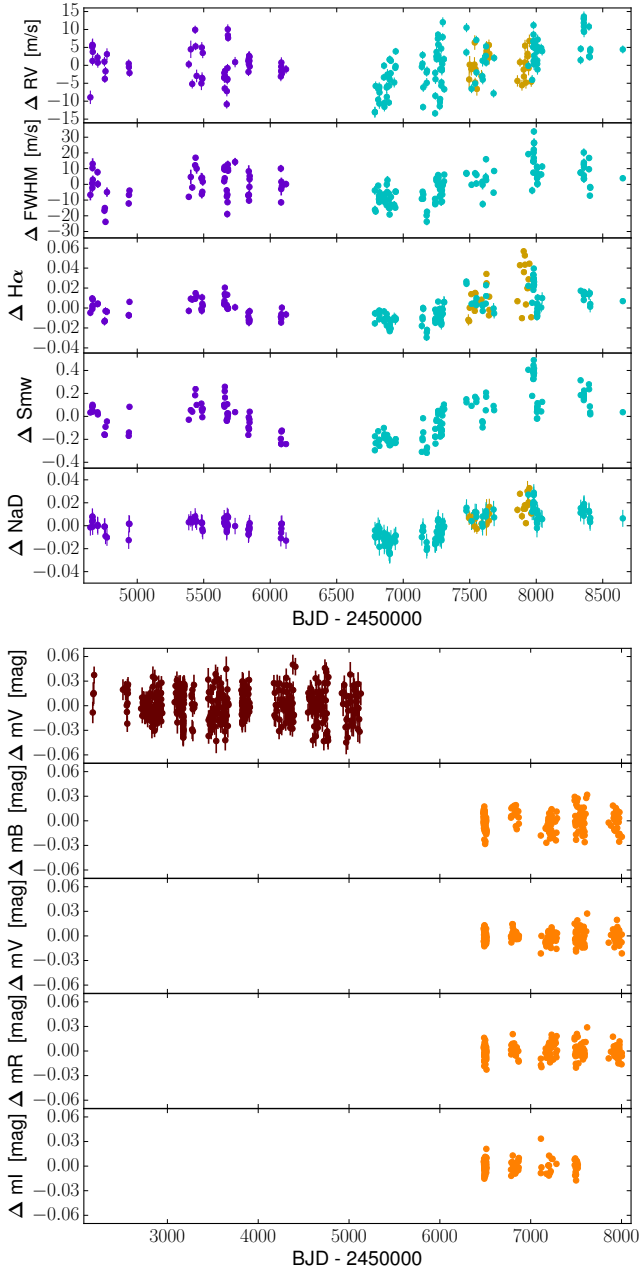
Fig. 1. Top: time series of the RV and the chromospheric activity indicators with combined measurements from HARPS (represented in violet), HARPS-N (represented in cyan), and CARMENES (represented in yellow). Bottom: time series of the photometric magnitudes taken with ASAS (represented in dark red) and EXORAP (represented in orange) in the B , V , R , and I filters.
