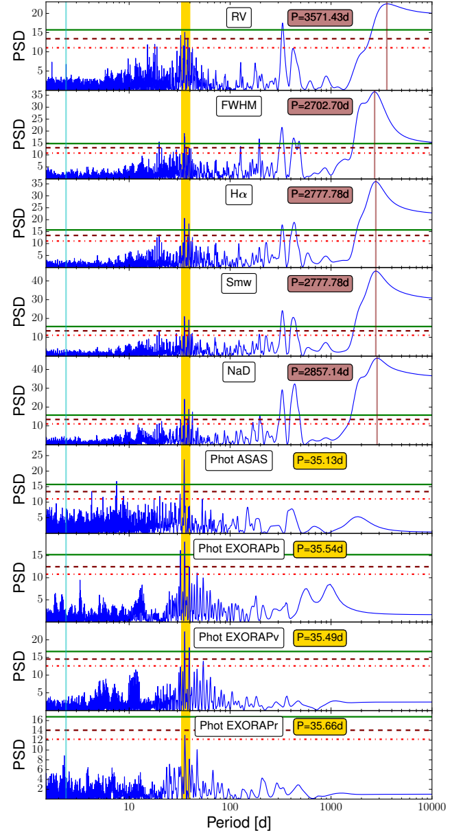
Fig. 2. Periodograms of the RV, FWHM, H\alpha , S_{\text{mw}} , NaD, ASAS V , EXORAP B , EXORAP V , and EXORAP R -band magnitude time series. The periods related to stellar rotation, planetary companion, and possible magnetic cycle have been represented as yellow, cyan, and brown vertical lines, respectively. The green, brown, and red horizontal lines indicate the 0.1, 1, and 10% FAP levels, respectively.
