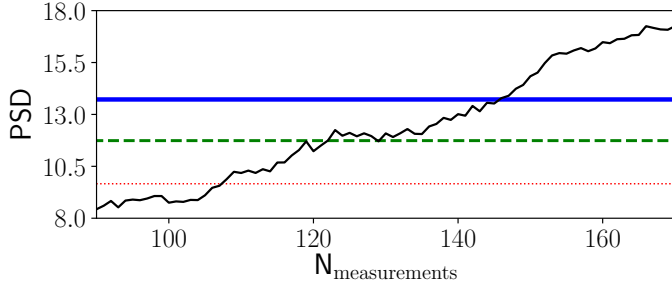
Fig. A.2. Evolution of the PSD associated with the planetary signal along the number of RV measurements considered. The blue, green, and red horizontal lines indicate the 0.1, 1, and 10% FAP levels, respectively.
