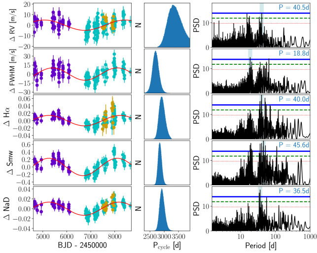
Fig. 3. Analysis of the long-term signal. Left: RV, FWHM, H\alpha , S_{mw} , and NaD time series with their respective model of the long-term signal. Center: posterior distribution for the periodicity of the long-term signal. Right: periodograms of the residuals after subtracting the model. The blue, green, and red horizontal lines indicate the 0.1, 1, and 10% FAP levels, respectively. The highest peak of the periodogram is marked with a blue shaded area.
