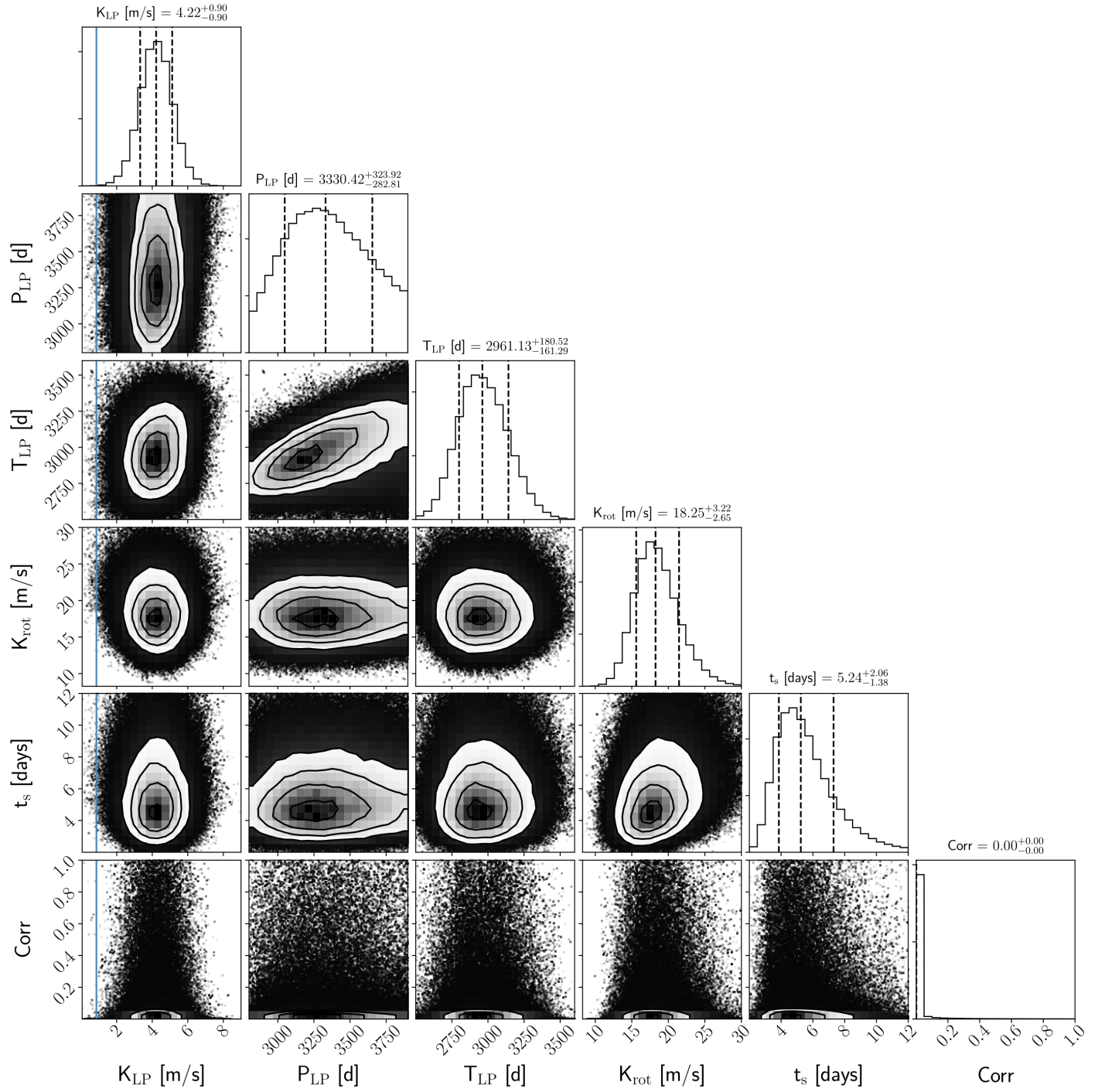
Fig. A.1. Posterior distributions of the cycle and rotation fitted parameters from the cycle+rotation+Keplerian model applied to the RV time series. The 16th–84th percentiles are represented through vertical dashed lines.
