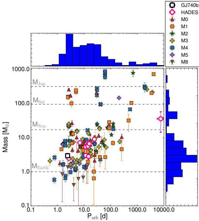
Fig. 8. Mass-period diagram including the detected exoplanets from NASA exoplanets archive with published masses and orbital periods orbiting around M-type stars. The sub-spectral type of the parent star is indicated with a unique symbol and color. GJ 740 b has been represented with an unfilled black square, and the HADES detections (GJ 3998 b and GJ 3998 c, Affer et al. 2016 ; GJ 625 b, Suárez Mascareño et al. 2017 ; GJ 3942 b, Perger et al. 2017a ; Gl 15 A b and Gl 15 A c, Pinamonti et al. 2018 ; Gl 686 b, Affer et al. 2019 ; Gl 49 b, Perger et al. 2019 ; and GJ 685 b, Pinamonti et al. 2019 ) have been marked with pink unfilled dots. The four horizontal dashed lines indicate the mass of Jupiter, Saturn, Neptune, and the Earth as a reference. The top and right panels contain the mass and orbital period distribution of the sample.
