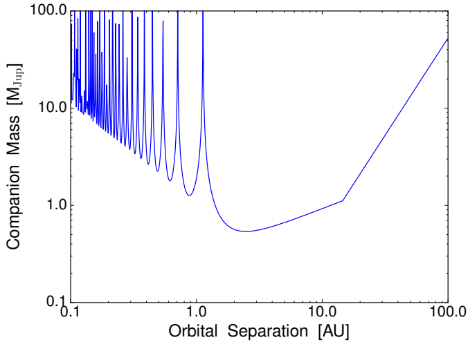
Fig. 10. Diagram of the minimum mass of a planetary companion for GJ 740 at different orbital radius based on the proper motion difference method.
