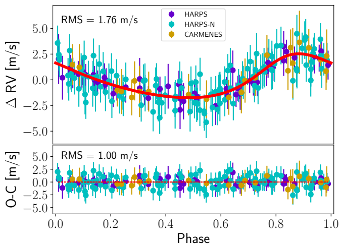
Fig. 7. Top: phase-folded curve of the RV time series using the GJ 740 b orbital period after subtracting the long-term signal and the rotation period. The jitter terms of each spectrograph have been added to the original RV errors. The red solid line represents the planetary model. Bottom: residuals after subtracting the model.
