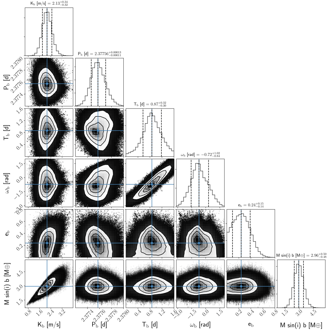
Fig. 6. Posterior distributions of the GJ 740 b fitted parameters. The 16th–84th percentiles are represented through vertical dashed lines.
