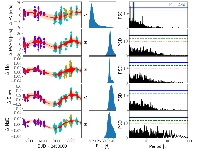
Fig. 4. Analysis of the rotation signal. Left: RV, FWHM, H\alpha , S_{mw} , and NaD time series with their respective model of the long-term signal and the rotation signal. The shaded regions indicate the 1\sigma confidence band of the GP model. Center: posterior distribution for the periodicity of the rotation signal. Right: periodograms of the residuals after subtracting the model. The blue, green, and red horizontal lines indicate the 0.1, 1, and 10% FAP levels, respectively. The highest peak of the periodogram is marked with a blue shaded area.
