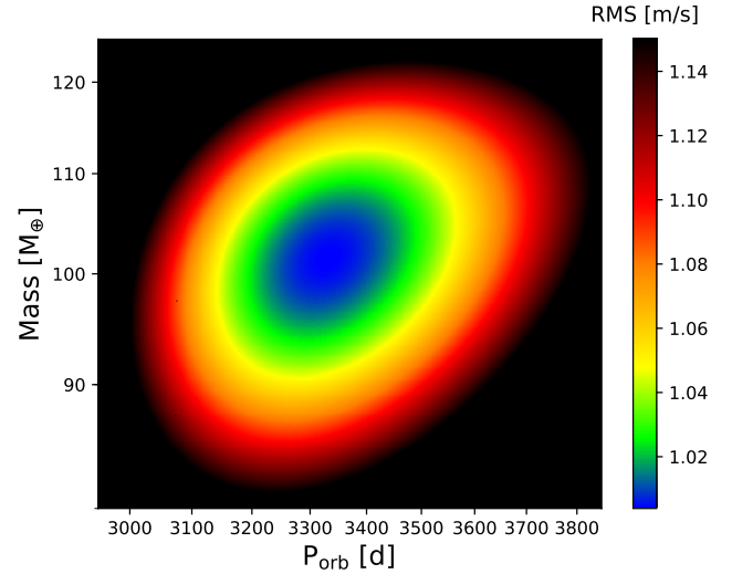
Fig. 9. Distribution of the RMS of the residuals in the RV time series after subtracting the long-term signal with a sinusoidal function whose amplitude is calculated from the considered values of mass and period.
