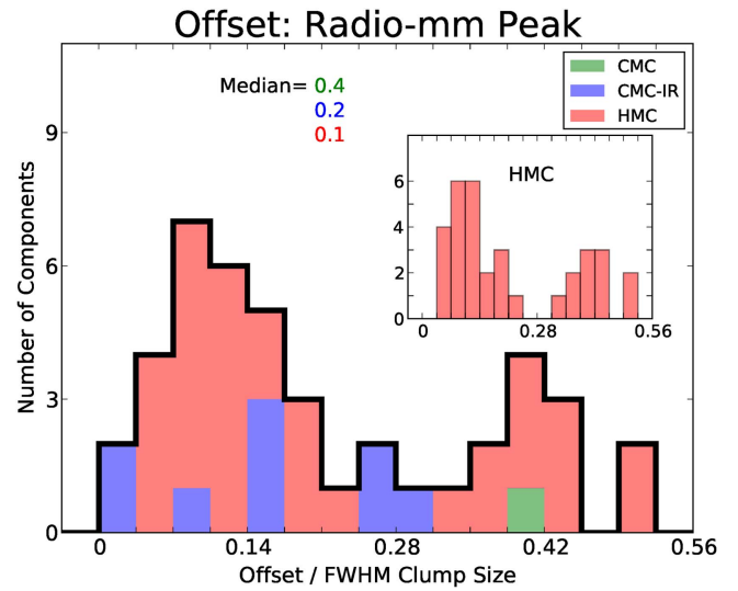
Figure 3. Position offsets between radio sources and the 1.2 mm peaks divided by the FWHM size of each clump. The inset shows the distribution only for the HMC detections. If no 1.2 mm data were available, we used the median FWHM size for the specific type of clump. The median FWHM sizes for each type of clump in this sample are 31'', 25'', and 18'' for CMCs, CMC-IRs, and HMCs, respectively. The average centimeter positional accuracy is better than 0.1'', and the typical positional accuracy for the 1.2 mm data is a few arcseconds. Clumps with multiple components (within a radius of 3'') have been treated as a single radio source in this histogram. Using a Kolmogorov-Smirnov test to analyze the spatial offset distribution of the HMCs and CMC-IRs, we estimated a p -value = 0.34. Thus, there is no strong evidence that these two distributions are different.
