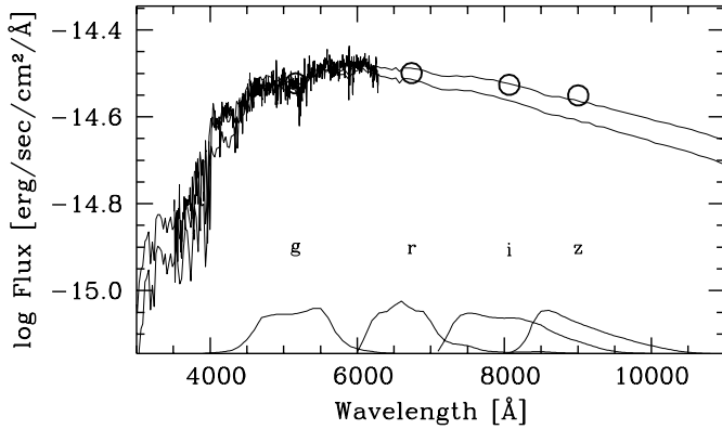
Fig. 5. Composite spectral energy distribution of galaxy N50. The CASLEO spectrum, in the range 3500 \leq \lambda \leq 4400 Å has been matched to ESO observations ( 4400 \leq \lambda \leq 6300 Å) while integrated g , r , i , and z Gunn magnitudes have been converted into monochromatic fluxes. Absolute flux calibration reproduces galaxy energy distribution within the central 15'' aperture. Two SSP models from Buzzoni (1989), with [\text{Fe}/\text{H}] = -0.25 and age 5 and 15 Gyrs, are superposed on the plot (thin solid lines, the older model is the “redder” one)
