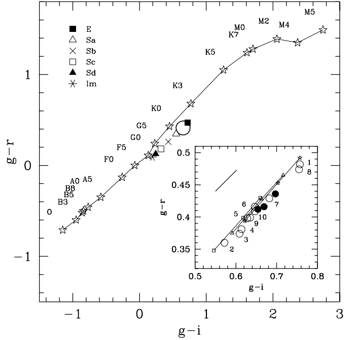
Fig. 4. ( Main panel ) – Two-colour diagram comparing N50 integrated g-r and g-i (big open dot) with the stellar Main Sequence from the Vilnius spectral atlas (star markers) and with Buzzoni’s (1998, 2000) 15 Gyr galaxy models for different Hubble types, as labelled top left. ( Insert panel ) – N50 aperture photometry (solid dots) and individual colours of the visible knots in the galaxy central region (open dots with identification labels according to Table 1). Aperture photometry is for circular spots at 2''.5 , 10'' , and 30'' from galaxy centre. Colours become bluer at larger distance. Buzzoni’s (1989) SSP evolutionary sequences for 5, 10, and 15 Gyr (in the sense of redder colours) are superposed (thin solid lines). Model metallicity is for [\text{Fe}/\text{H}] = -0.25 (squares), 0.0 (triangles) and +0.3 (stars). A reddening vector for E(B-V) = 0.03 mag is displayed top left in the panel
