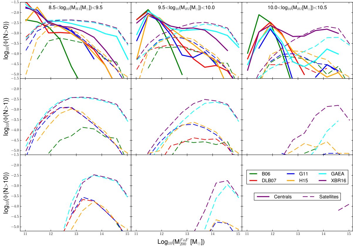
Figure 9. Mass function of FoF haloes hosting at least one (top panel), more than one (middle panel), and more than ten (bottom panel) galaxies with HI mass in different bins (different columns). Solid lines are used for central galaxies while long-dashed lines correspond to satellite galaxies.
