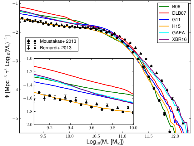
Figure 2. The galaxy stellar mass function predicted by the six models used in our study, compared to observational measurements by Moustakas et al. (2013, circles) and Bernardi et al. (2013, triangles), both based on SDSS. The inset shows a zoom on the low-mass end.
