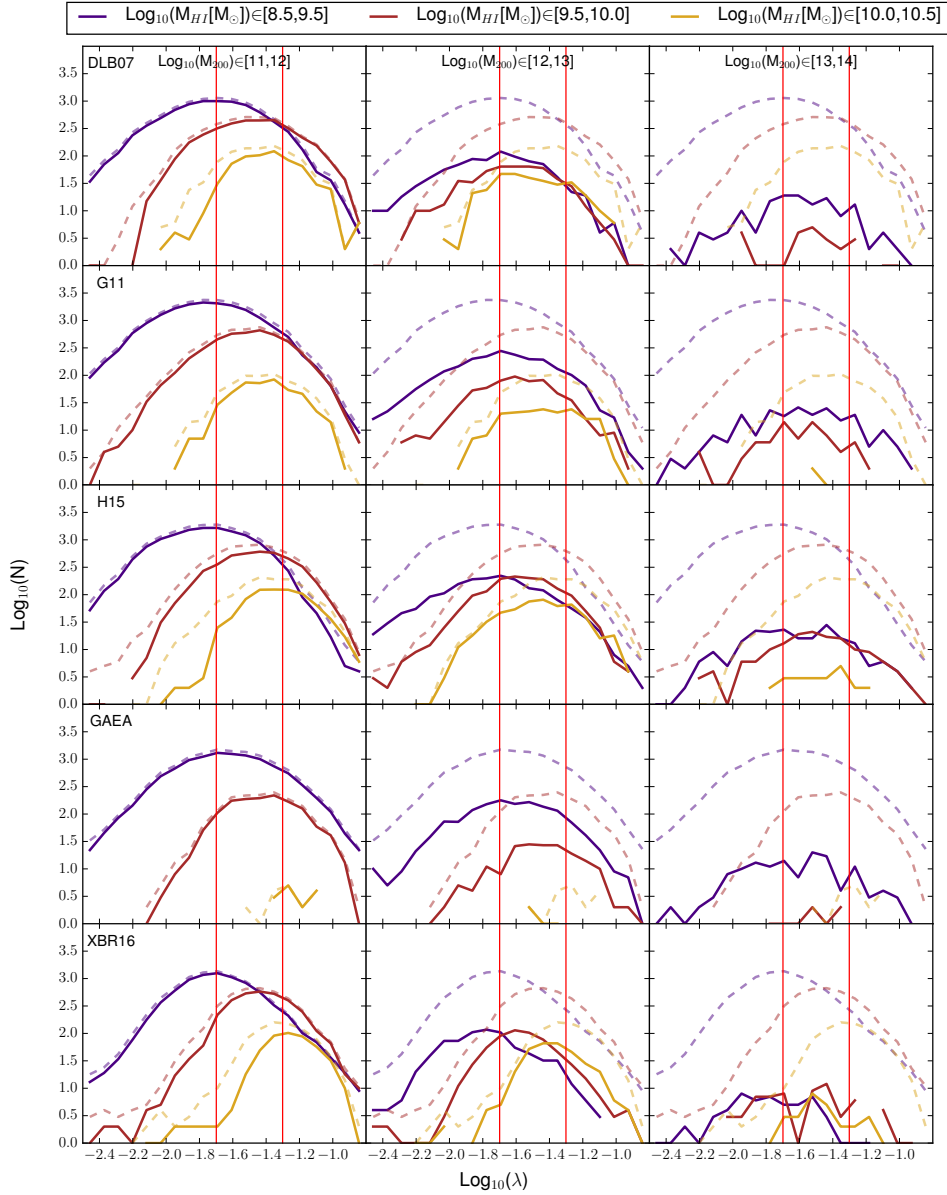
Figure 15. Distribution of halo spin values for galaxies selected in haloes with different M_{200}^{max} (columns) and HI mass (same colours of Fig. 6), for all models used in our study (different rows). The solid lines represent the distribution for each selection, while dashed lines are the total distribution over all the M_{200}^{max} range, reproduced in every panel as reference. The vertical red lines show the spin division considered by P13, and are plotted as reference.
