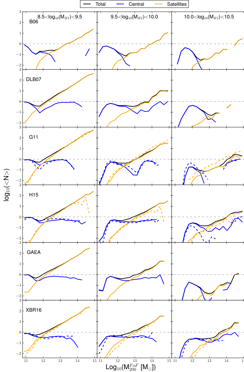
Figure 8. Average number of galaxies with stellar mass larger than M_* > 10^9 M_\odot and in different HI mass bins (different columns) for haloes of mass M_{200}^{FoF} . Different rows correspond to the different models considered in our study. The colour coding is the same as in Fig. 4: black for all model galaxies, blue for centrals and orange for satellites. In the rows corresponding to the G11, H15 and the XBR16 models, the dashed lines correspond to results based on the MS-II simulation.
