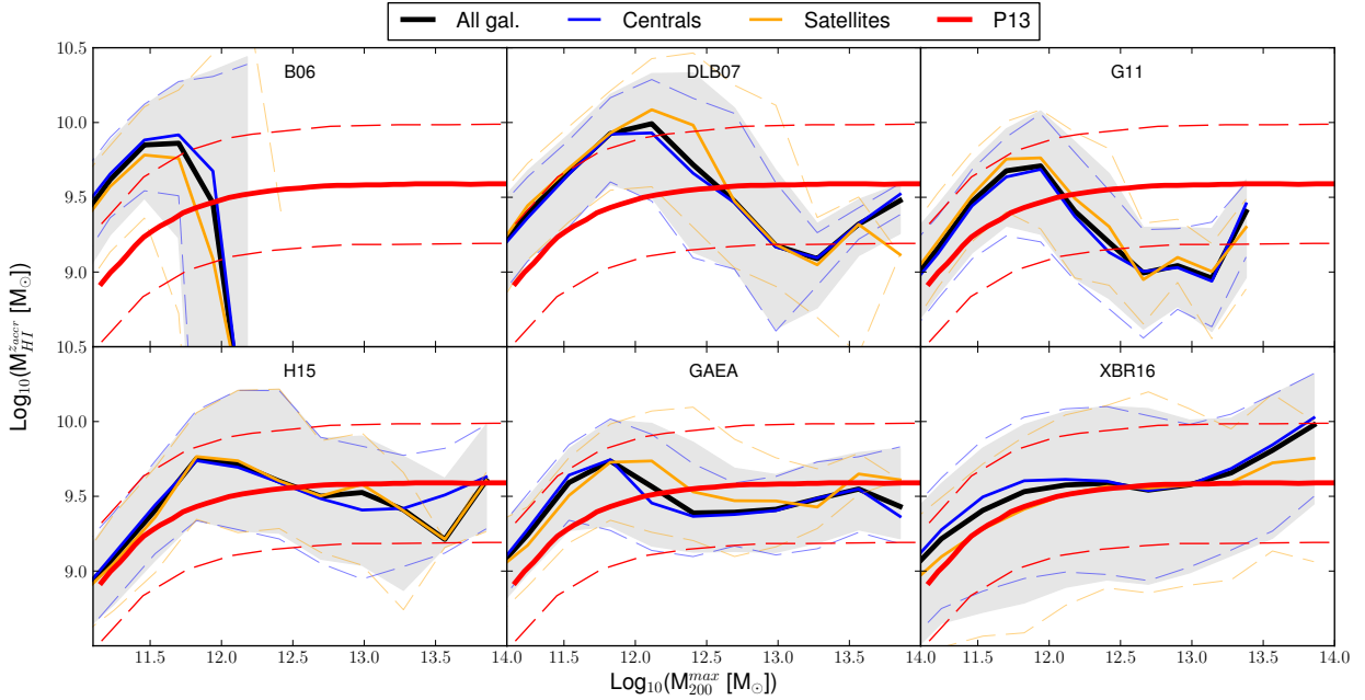
Figure 13. The HI-halo mass relation for the models considered in this study, for central (blue), satellite (orange) and all (black) galaxies. The relation inferred by P13 is shown for comparison (red). The HI mass shown on the y axis is that measured at the time the parent halo mass peaks (i.e. just before infall). Solid lines show the median values, shaded region corresponds to the 1\sigma scatter for all galaxies, while dashed lines correspond to the 1\sigma scatter for centrals and satellites.
