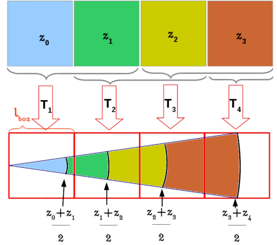
Figure 1. A schematic illustration of our light-cone construction algorithm: a grid of cubic boxes with size length l_{box} (red) is built over the cone, and galaxies inside each box of the grid are randomly shifted/rotated/inverted depending on the specific box they end up in. Galaxies are extracted from the simulation output with redshift closest to the co-moving distance to the observer.
