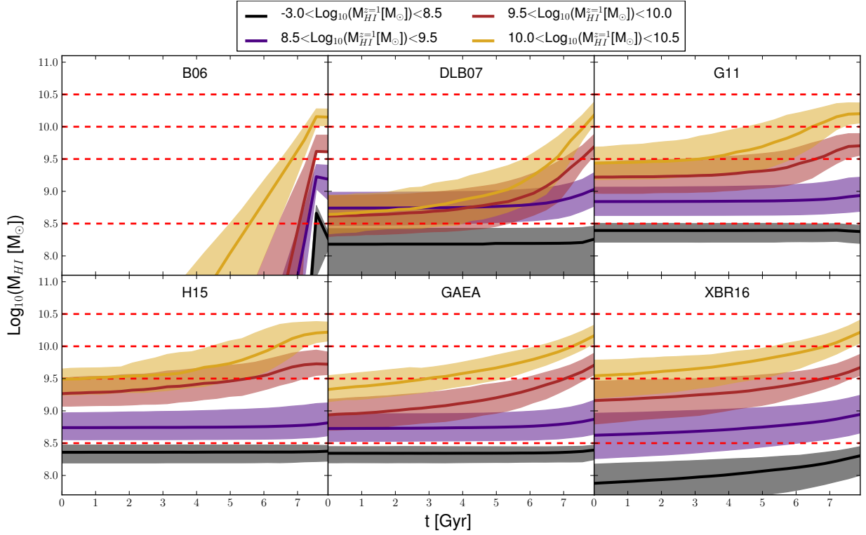
Figure 12. The HI content of satellites accreted at redshift 1 vs the look-back time. Galaxies are divided according to their initial HI content, with different colours representing different HI mass bins at z=1 . The solid lines correspond to the median of the distributions, while the shaded areas show the one sigma scatter. The red dashed lines correspond to the limits of the HI mass bins considered, and are plotted as a reference.
