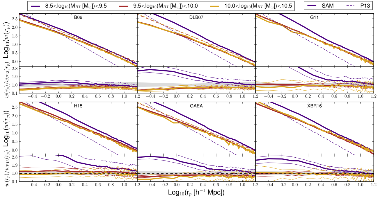
Figure 6. The two-point projected correlation function for different bins in HI mass (solid thick lines of different colours). Each panel corresponds to a different model, and the lower sub-panels show the ratio between the model predictions and the corresponding observational estimates (dashed lines) by P13 for the medium HI mass bin. As discussed in the text, this is equal to the one of the highest HI mass bin and more reliable than the measurements corresponding to the lowest HI mass bin. The 1\sigma scatter is shown in the lower sub-panels using thin lines for models and a shaded region for the data.
