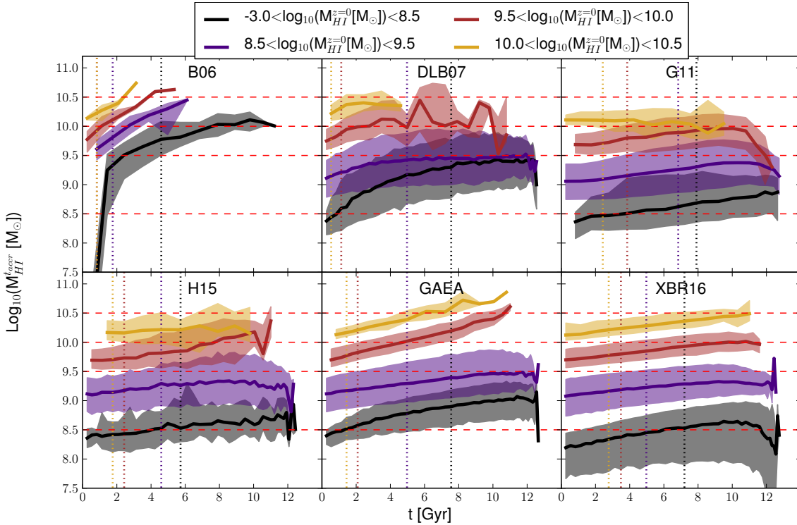
Figure 11. The HI content of satellites at the time of accretion vs the look-back time of accretion. Galaxies are divided according to their final HI content, with different colours representing different HI mass bins. The solid lines correspond to the median of the distributions, while the shaded areas show the one sigma scatter. The vertical dotted lines are the median times of accretion of model galaxies in each HI bin (colour coded as above). The red horizontal dashed lines correspond to the limits of the HI mass bins considered, and are plotted as a reference.
