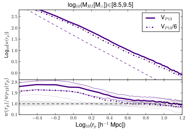
Figure 7. The 2PCF for the lowest HI mass bin for the XBR16 model. The solid line corresponds to model predictions for the full volume considered (i.e. this line corresponds to that shown in Fig. 6). The dot-dashed line corresponds to the results obtained when considering only one sixth of the volume, as in the observational sample by P13. In the lower sub-panel, we show the ratio between model predictions and the observational estimate of the medium HI bin. Shaded regions and thin lines show the 1\sigma scatter.
