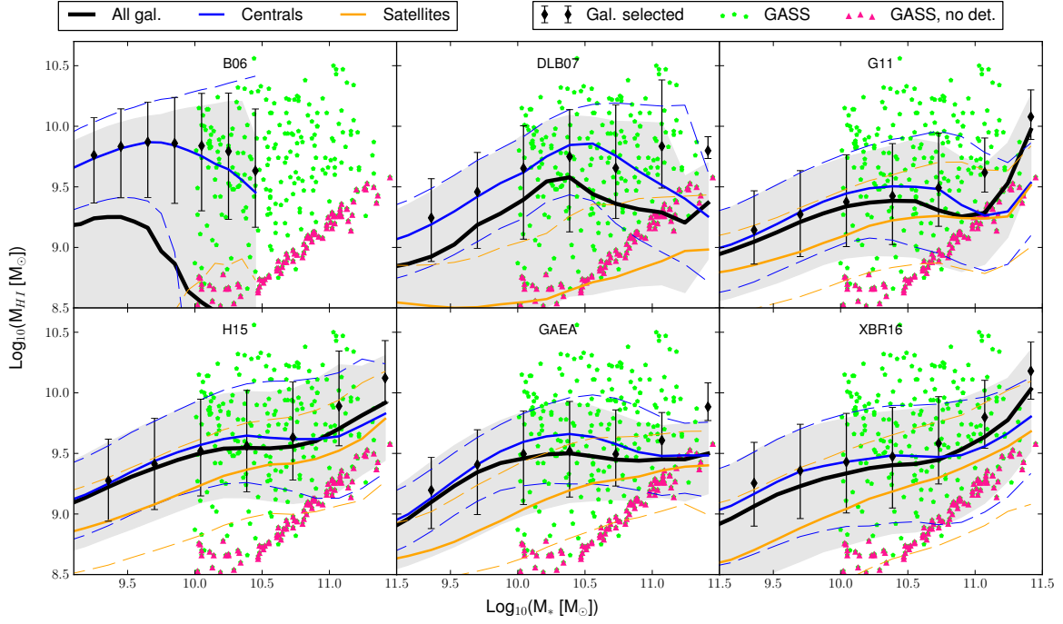
Figure 4. The predicted relation between HI mass and galaxy stellar mass, compared to results from the GALEX Arecibo SDSS Survey (symbols). Lines of different colours are used for central galaxies (blue) and satellites (orange), while the black lines and shaded regions correspond to the entire galaxy population. Solid lines correspond to the median of the distributions, while dashed lines (and the shaded region) mark the 1\sigma distribution. The black diamonds with error-bars show the distribution of all model galaxies when using the same detection threshold of the data. Symbols of different colours are used for detections (green pentagons) and non detections (upper limits, purple triangles).
