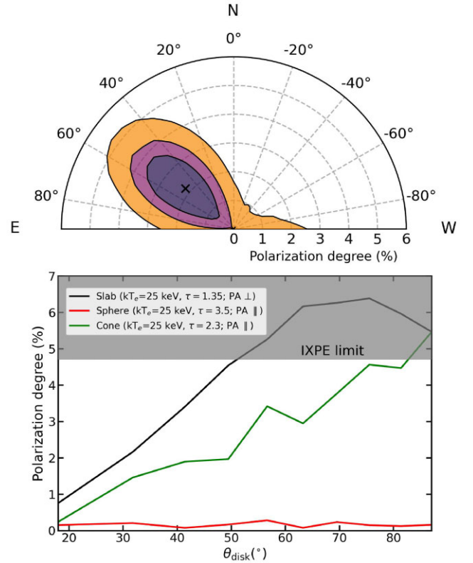
Figure 3. Top-panel: contour plot of the polarization degree \Pi and angle \Psi associated to the primary power law component. Purple-, pink-, and orange-shaded regions indicate 68 per cent, 90 per cent, and 99 per cent confidence levels for two parameters of interest, respectively. Bottom-panel: Monte Carlo simulations performed with the Comptonization code MONK. The input coronal parameters kT_e , \tau correspond to the spectral shape reported in Table 1 and the polarization angle is reported with respect to the accretion disc plane.
