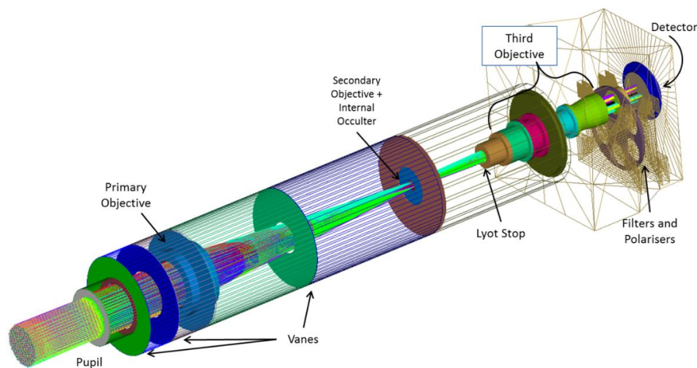
Figure 3 - Mechanical Model
