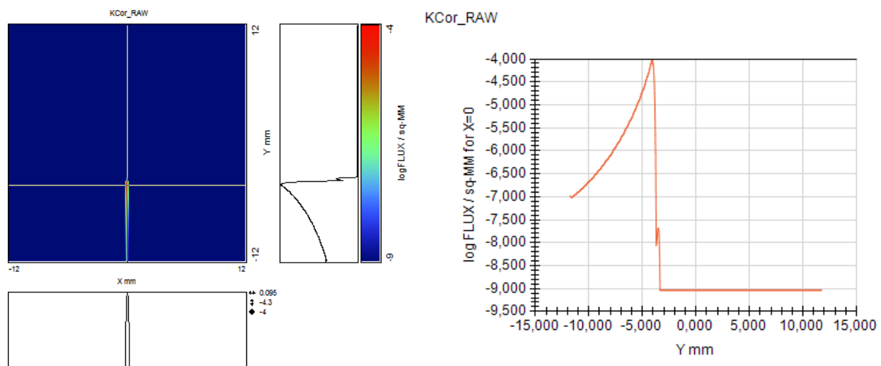
Figure 12. Propagation of the coronal signal inside ASPICS without degradation
