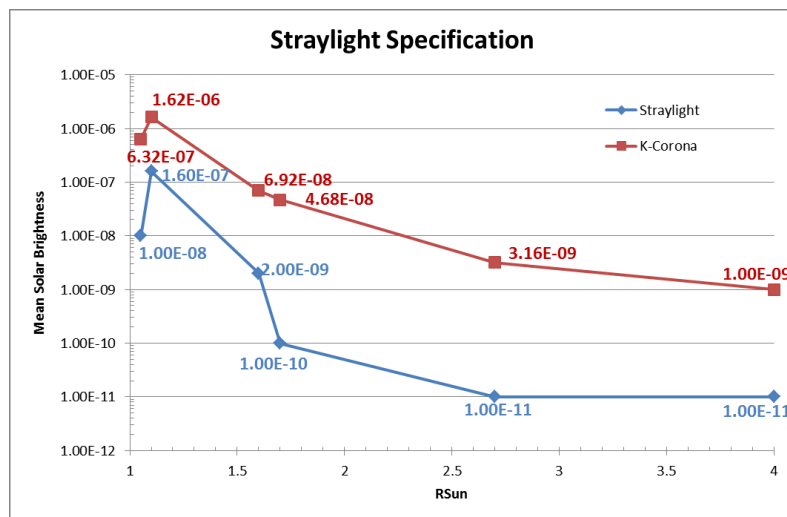
Figure 8 - Straylight Specification
