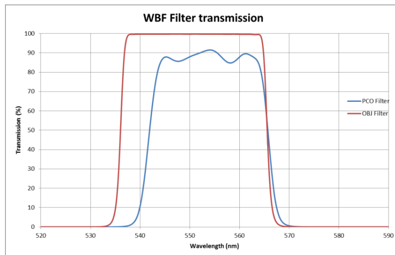
Figure 5 - Comparison of previous and new WBF transmission.
