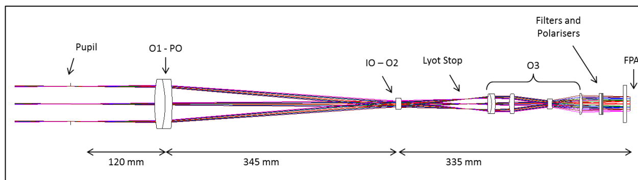
Figure 2 - Optical Model v15.2
