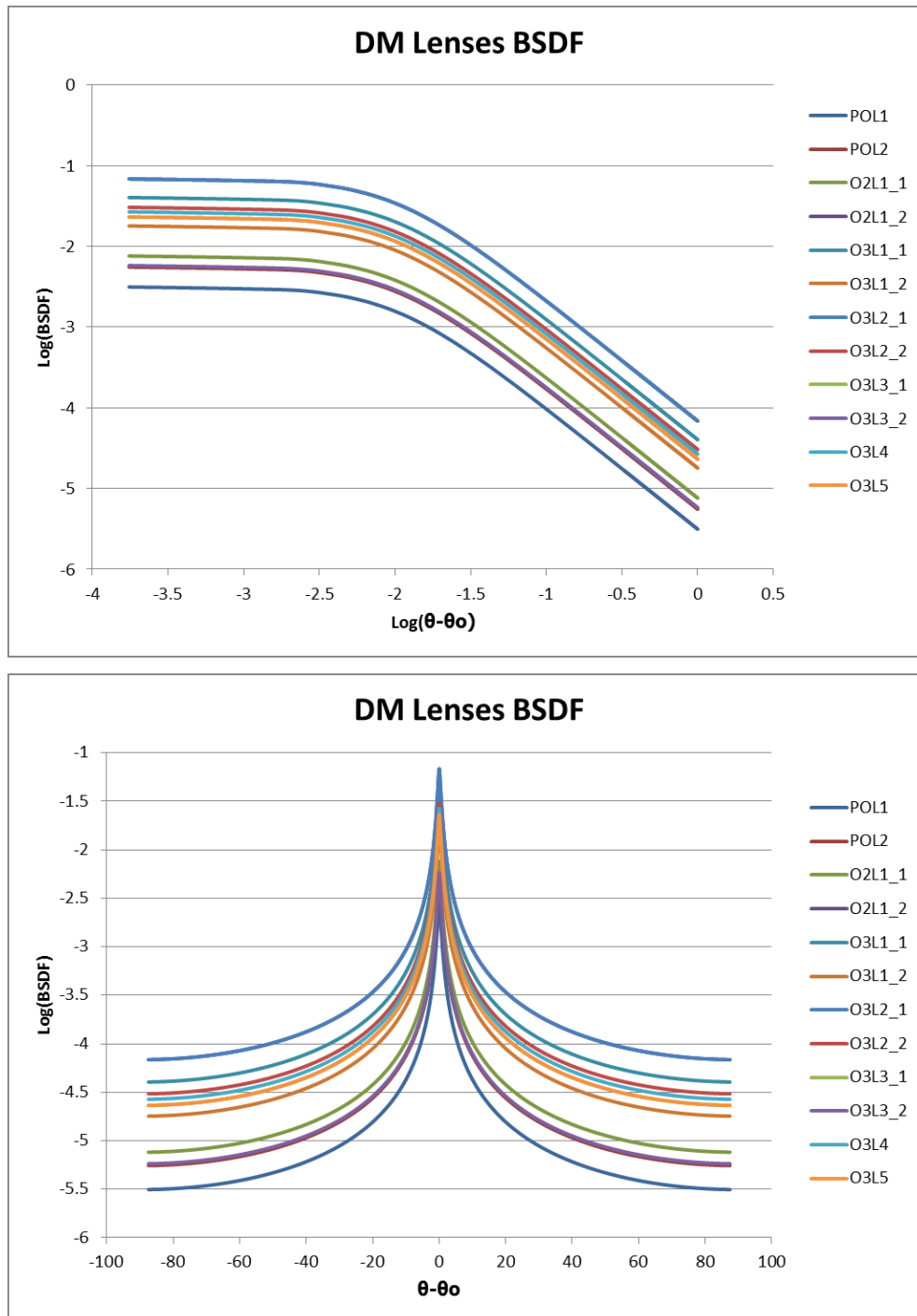
Figure 17. DM lenses log(BSDF) versus log(angle) (Up) and Log(BSDF) versus angle (down)
