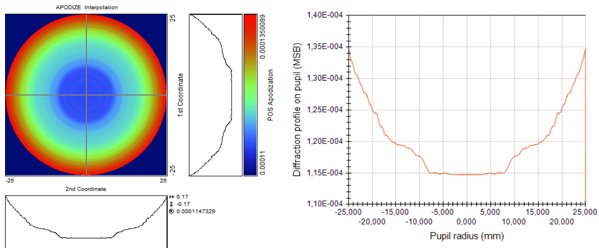
Figure 28. Pupil apodisation with diffraction profile
