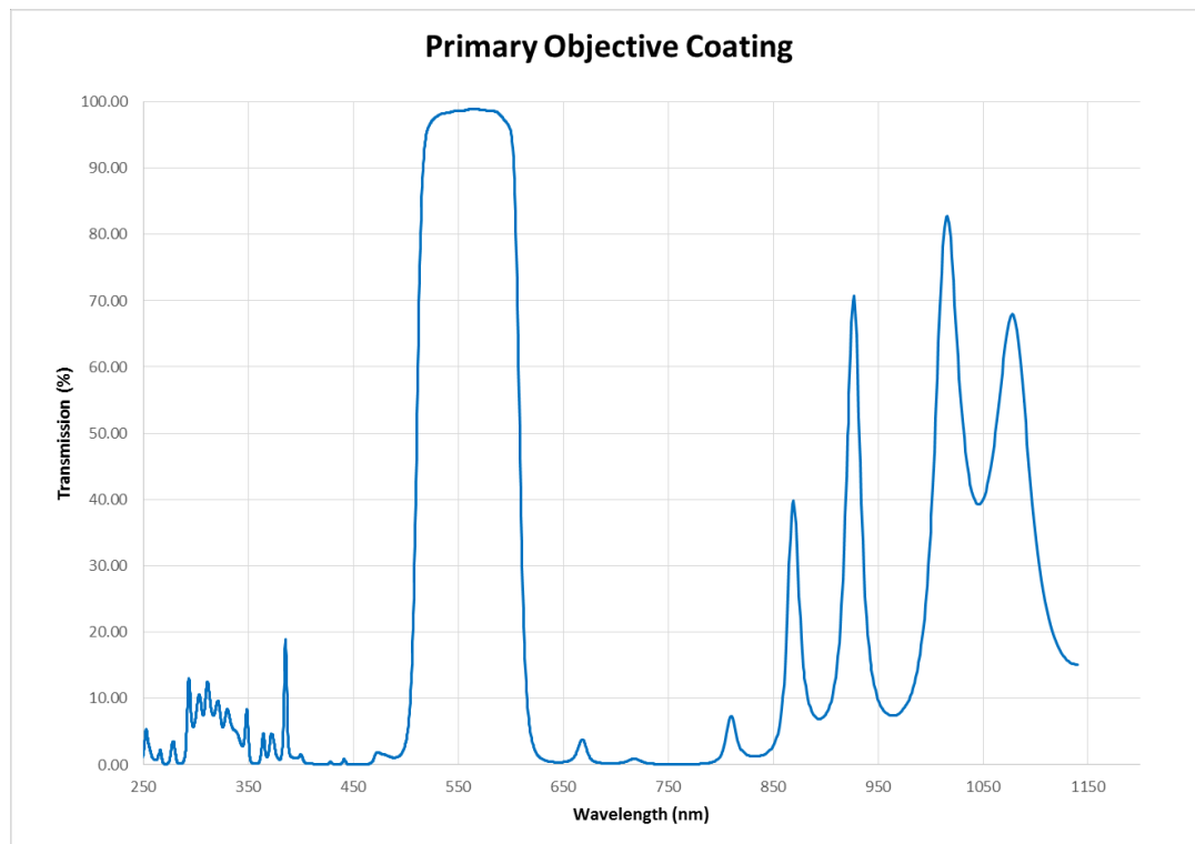
Figure 16. Primary Objective Coating transmission
