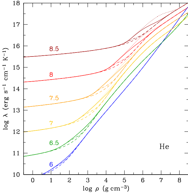
Fig. 2. Thermal conductivity for helium as a function of mass density for several constant temperatures T . The meaning of the various lines is the same as in Fig. 1.
