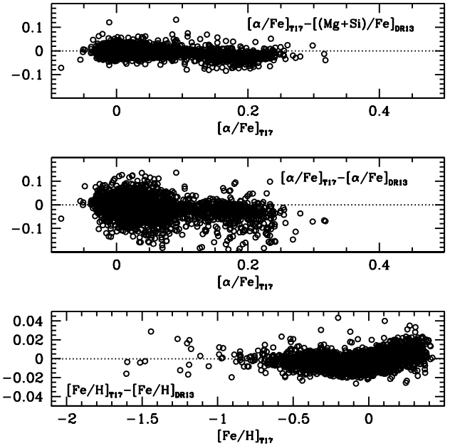
Fig. 7. Bottom panel: difference between [Fe/H] values adopted by T17 ( [Fe/H]_{\text{T17}} ) and [Fe/H] as listed in the DR13 catalogue ( [Fe/H]_{\text{DR13}} ), as a function of [Fe/H]_{\text{T17}} . Middle panel: same as bottom panel, but for [\alpha/Fe] , considering the total \alpha -enhancement from DR13 data (see text for details). Top panel: same as middle panel, but in this case the DR13 estimate is actually [(Mg + Si)/Fe] (see text for details).
