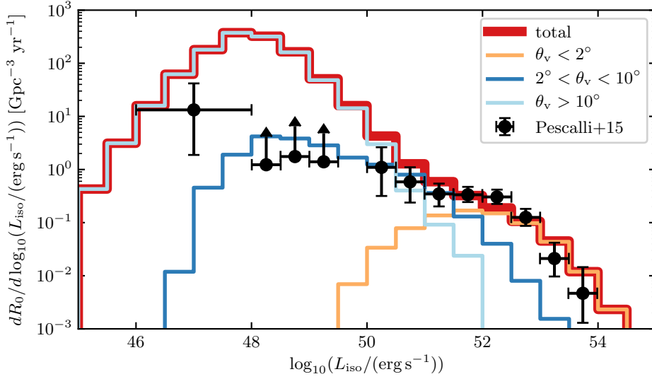
Fig. 4. LGRB luminosity distribution of our model population (thick solid red histogram) compared to the observed distribution (black points, from Pescalli et al. 2015). Thinner histograms show the luminosity distributions of three sub-classes corresponding to three viewing angle bins, reported in the legend.
