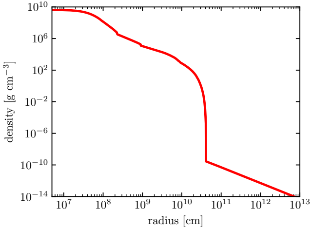
Fig. 2. Radial density profile from our representative LGRB progenitor (model 16TI of Woosley & Heger 2006), which represents a low-metallicity, high-angular momentum, massive star prior to collapse. The low-density power-law tail, visible in the lower-right corner of the figure, has been added by ourselves to the original density profile of the model. It represents a stellar wind with typical Wolf-Rayet mass loss rate \dot{M}_w = 10^{-5} M_\odot \text{ yr}^{-1} and velocity v_w = 1000 \text{ km s}^{-1} .
