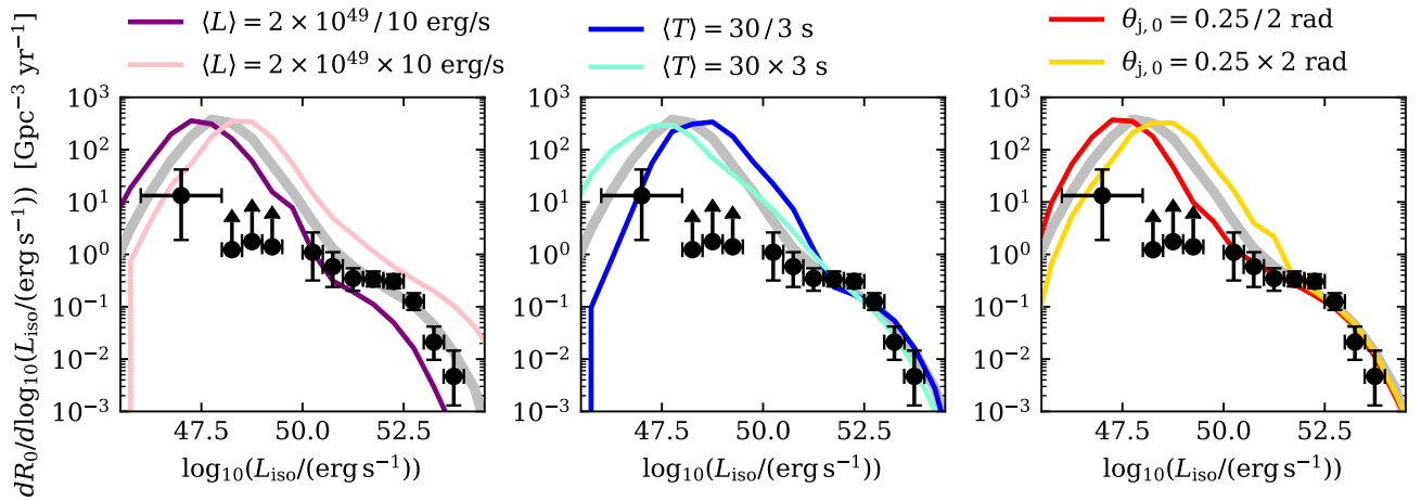
Fig. 5. Long GRB luminosity function dependence on the parameters of the jet at launch. Each panel shows how the fiducial luminosity function (thick grey solid line) is affected by a change in one of the parameters (coloured thinner lines). See text for an interpretation of the dependencies.
