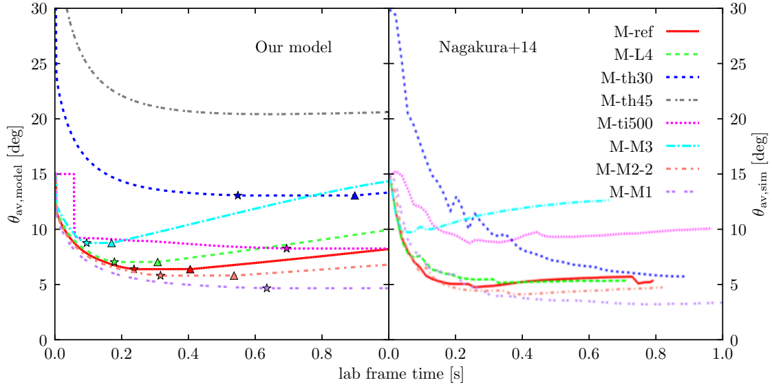
Fig. A.1. Comparison between the height-averaged opening angle evolution from the numerical simulations in Nagakura et al. 2014 ( right-hand panel , adapted from their Fig. 3) and those predicted by our semi-analytical model ( left-hand panel ). Each line refers to a different initial configuration (see text). Stars and upward triangles in the left-hand panel mark t_{bo} and t_{bo} + t_{delay} (see Sect. 3), respectively. The evolution for configuration M-th45 is not shown in the original figure.
