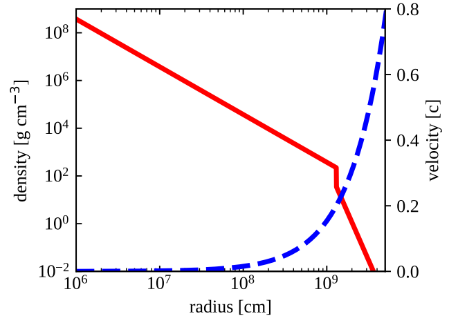
Fig. 6. Density and velocity profile of the SGRB ambient medium model. The red line shows a snapshot of the density profile (along the polar axis) of the neutron star merger ejecta model described in Xie et al. (2018) (also used in Kasliwal et al. 2017 and Gottlieb et al. 2018b). The blue dashed line shows the corresponding velocity profile (velocity axis on the right). The ejecta are assumed to expand homologously.
