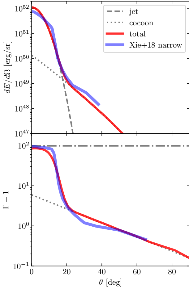
Fig. A.3. Same as Fig. A.2, but for the “narrow engine” case in Xie et al. (2018) (we choose the structure extracted from the 10^4 s snapshot as shown in their Fig. 2, right-hand panels).
