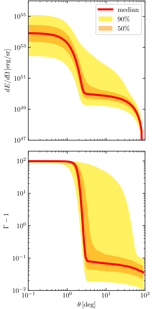
Fig. 3. Distribution of jet structures in our LGRB population. In each panel, at each fixed angle \theta , the yellow (resp. orange) filled area encloses 90% (resp. 50%) of the structures in the population, while the red line shows the median of the distribution at that angle. Top panel: energy structures (kinetic energy per unit solid angle as a function of the angle \theta from the jet axis). Bottom panel: velocity structures (average Lorentz factor diminished by one, as a function of \theta ).
