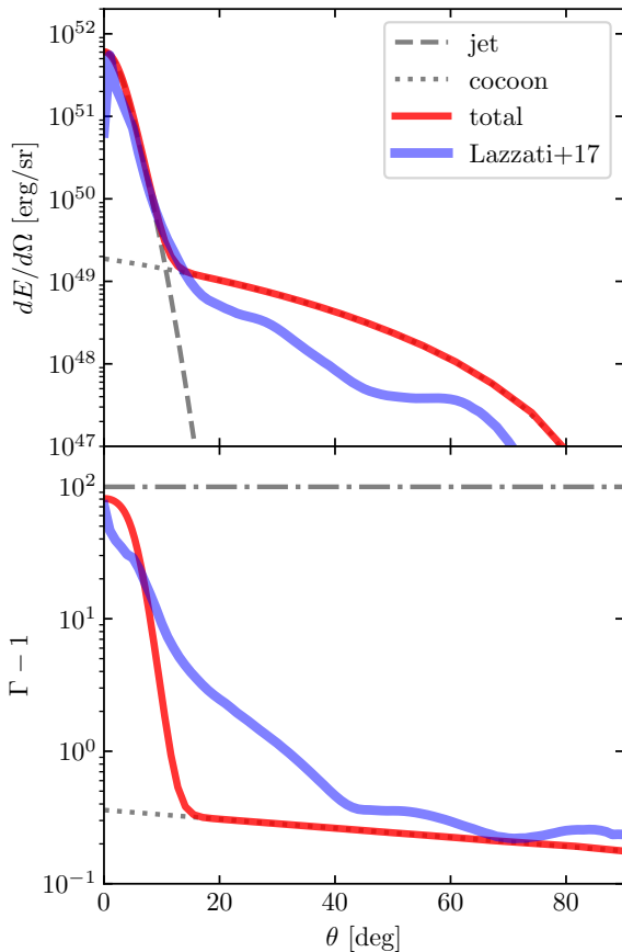
Fig. A.2. Comparison between the jet structure predicted by our model and the results of numerical simulations by Lazzati et al. (2017b). Upper panel : distribution of kinetic energy per unit solid angle, while Lower panel : average Lorentz factor diminished by one. Grey dashed and dotted lines represent the jet and the cocoon as computed by our model (Sects. 3, 4 and 4.2). Red lines show the combined structure. Blue thick lines show the results of the numerical simulations (the Lorentz factor profile is given in Lazzati et al. 2018).
