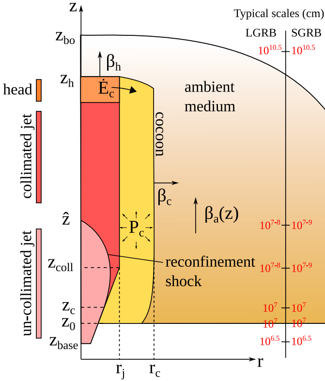
Fig. 1. Sketch of the various components of the jet propagation model, with some key quantities annotated. All quantities are defined and described in the text. Typical radii (order of magnitude in cm) are shown in red on the right, corresponding to the progenitors and average jet properties we employ when computing our synthetic jet populations (note that the collimation-related radii z_c , z_{coll} and \hat{z} change during the jet propagation).
