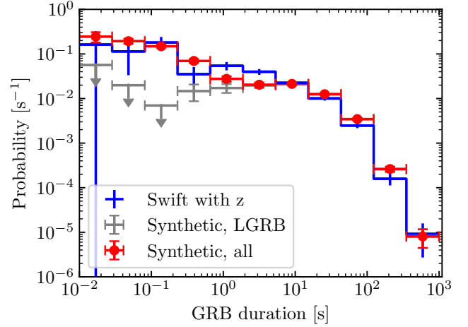
Fig. 11. GRB duration probability distribution. The blue histogram shows the estimated probability distribution of intrinsic duration (defined as T_{90}/(1+z) ) of Swift -detected GRBs with a measured redshift. Red points represent the corresponding distribution for our simulated populations (assuming an observed rate ratio of 13.5 between LGRB and SGRB, i.e. the same rate ratio as in the Swift sample), while the grey points show the distribution for the LGRB synthetic population alone (downward arrows are upper limits that correspond to empty bins). Vertical error bars show the Poisson uncertainty associated to each bin.
