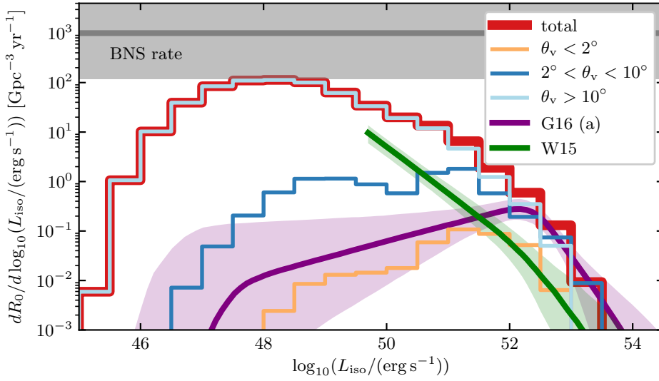
Fig. 8. SGRB luminosity distribution of our model population (thick solid red histogram) compared to two luminosity function models based on observations (Wanderman & Piran 2015 – green solid line and shaded area – and Ghirlanda et al. 2016 – purple solid line and shaded area). Thinner histograms show the luminosity distributions of sub-classes of jets belonging to three viewing angle bins, reported in the legend. The grey line and filled horizontal band show the binary neutron star merger local rate based on gravitational wave observations (The LIGO Scientific Collaboration 2019).
