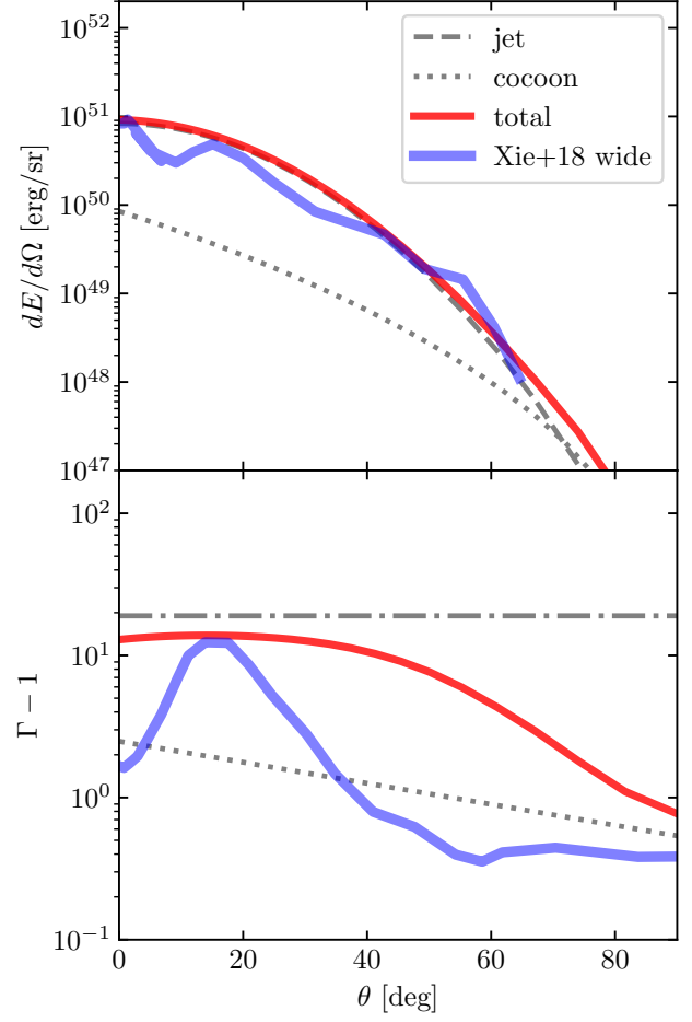
Fig. A.4. Same as Fig. A.2, but for the “wide engine” case in Xie et al. (2018) (we choose the structure extracted from the 10^4 s snapshot as shown in their Fig. 7, right-hand panels).
