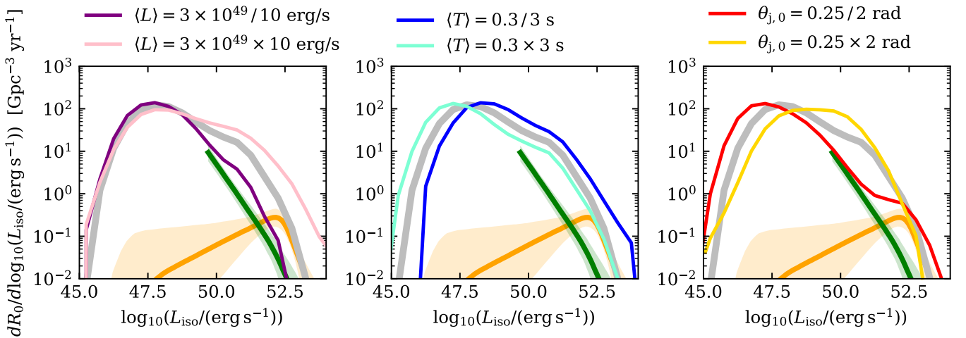
Fig. 9. Short GRB luminosity function dependence on the parameters of the jet at launch. In each panel, the thick grey line shows the synthetic short GRB luminosity function with fiducial parameters. The thinner, coloured lines show the impact of changing a single parameter. See text for a description of the various dependencies.
