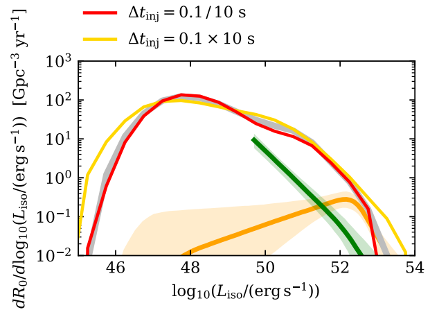
Fig. 10. Short GRB luminosity function dependence on the delay \Delta t_{\text{inj}} between merger and jet injection.
