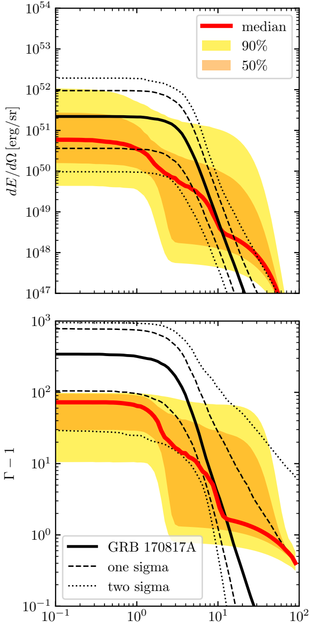
Fig. 7. Distribution of structures in our SGRB population. The filled areas and the red lines have the same meaning as in Fig. 3. The black lines show the confidence regions (dotted: two sigma, dashed: one sigma, solid: best fit) for the jet structure of GRB 170817A from Ghirlanda et al. (2019).
