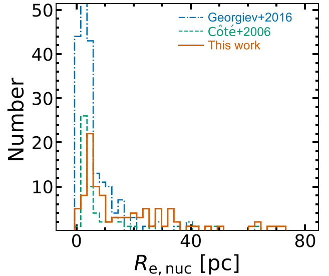
Figure 3. Comparison of the distribution of our 1D major-axis effective (half-light) radii of the nuclei (solid orange histogram) and previous circular effective radii of nuclei from Côté et al. (2006), dashed green histogram, and Georgiev et al. (2016), dash-dotted blue histogram.
