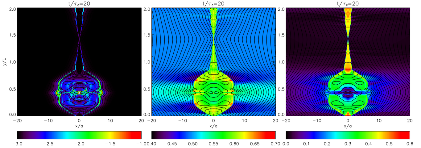
Figure 6. Images of various quantities at t = 20\tau_c , corresponding to the situation in the right-hand panel of Fig. 5. From left to right: the quantity |E \cdot B| in logarithmic scale (saturated for 10^{-3} and 10^{-1} , the maximum is \simeq 0.25 ); the plasma temperature p/\rho ; the magnitude of the velocity |v| . We recall that S = 10^6 , hence a = 0.01L .
