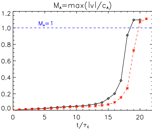
Figure 7. The maximum value over the spatial domain of the Alfvén Mach number M_A = |v|/c_A as a function of time, where the Alfvén speed c_A refers to the background, unperturbed value of 0.5. The solid black line (with diamonds) refers to the force-free equilibrium run, the red dashed line (with asterisks) refers to the pressure equilibrium run, and the blue dashed line indicates the threshold for super-Alfvénic flows.
