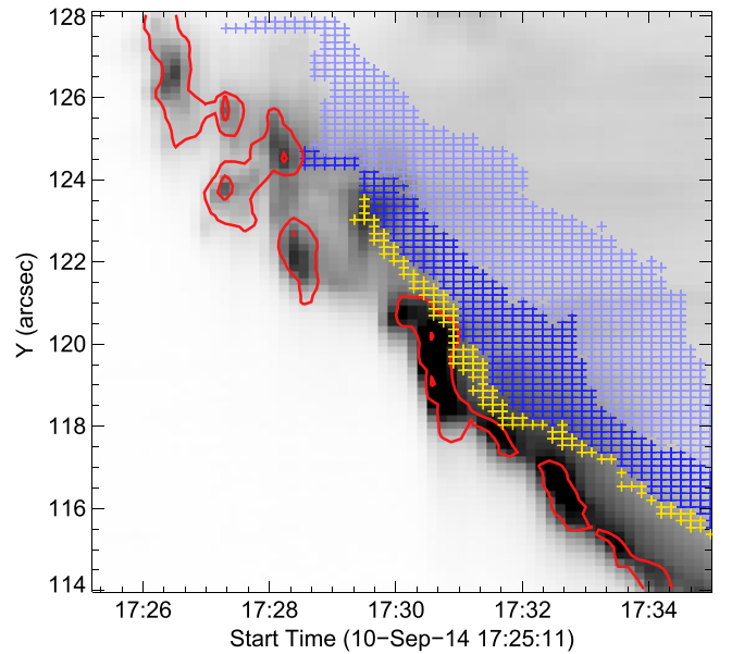
Figure 3. Mg II intensity spacetime map (inverted B/W color table) with overlays of Mg II downflows at the 30% bisector level at 15 and 30 \text{km s}^{-1} (red contours). The Fe XXI upflow velocities above 270, 200, and 100 \text{km s}^{-1} are indicated with yellow, dark blue, and light blue crosses, respectively.
