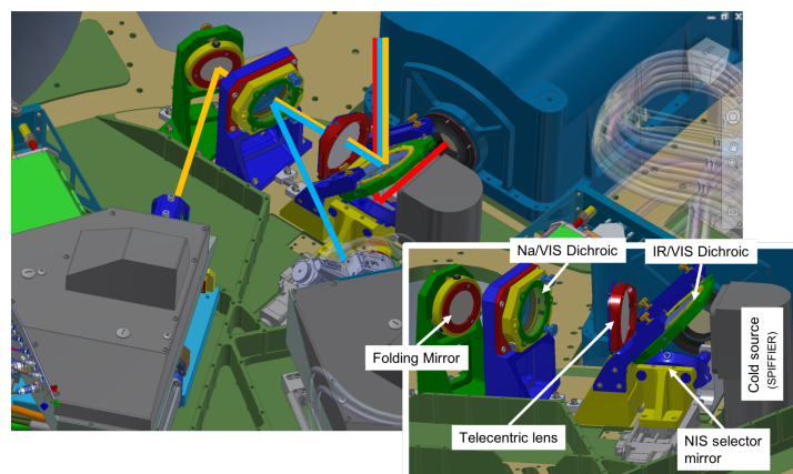
Figure 3. ERS Warm Optics
