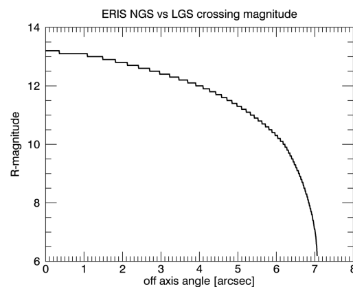
Figure 8 Transition magnitude vs NGS off-axis angle. Below the curve NGS-mode performs better than LGS-mode; the opposite above the curve.
