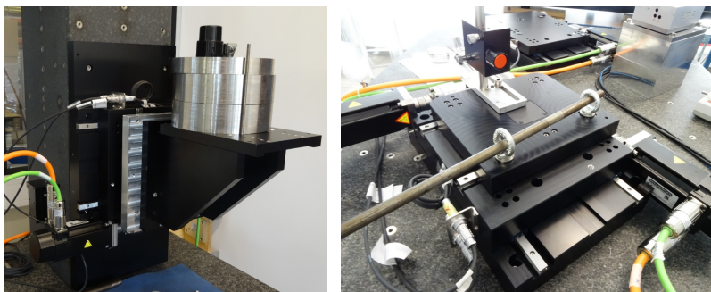
Figure 11. NGS WFS stage under vertical full-load test (Left) and under interferometric flexure testing (Right) during the acceptance test in Steinmeyer GmbH premises.
