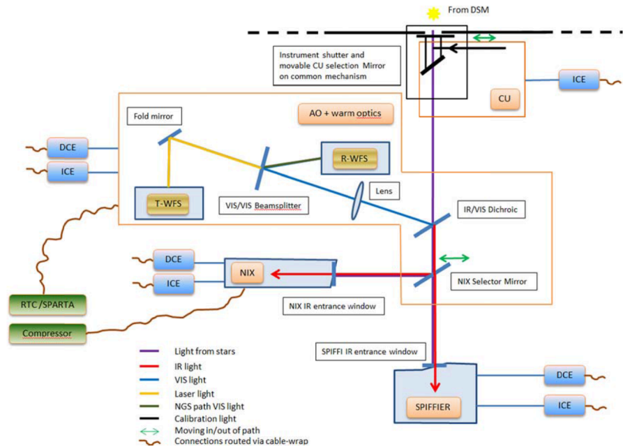
Figure 2 ERS instrument scheme
