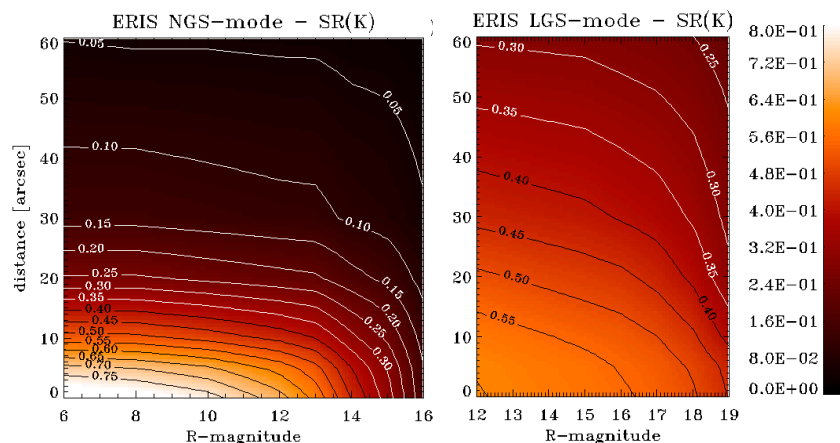
Figure 7 SR vs. NGS off-axis and mag. Left: NGS-mode; Right: LGS-mode
