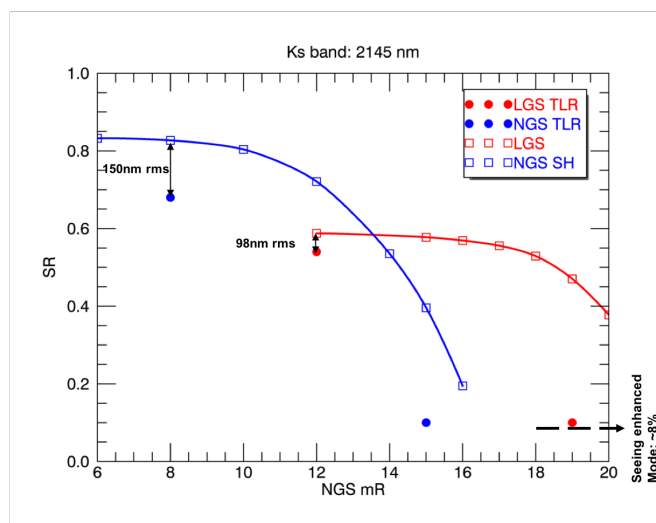
Figure 6 Estimated performance in Ks-band of the ERIS AO system
