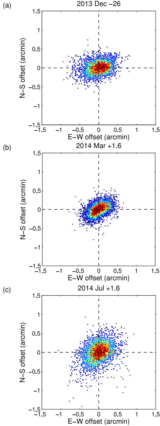
Figure 5. Position offsets for sources in the (a) 2013 Dec –26, (b) 2014 Mar +1.6 and (c) 2014 Jul +1.6 data sets, measured with respect to the time-averaged position of the source. The x -axis points west and the y -axis points north. The dotted lines mark the location of the origin. Points are coloured according to the local density on the page to show the shape of the distribution. Only one in five points is plotted.
