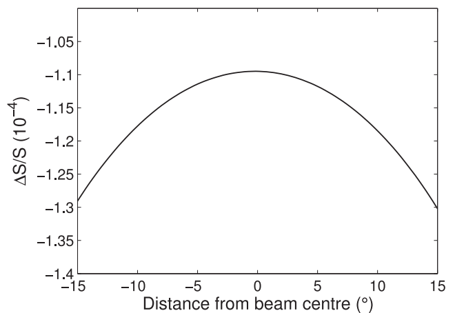
Figure 10. The predicted fractional deviation in peak flux density (compared to the true peak flux density) of a source as a function of position across the FoV for a zenith drift scan, due to a smooth ionosphere located at a constant altitude of 300 km. This calculation assumed an integration time of 112 s, an observing frequency of 154 MHz, a background TEC of 10 TECU and a PSF width of 130 arcsec, with the source passing directly overhead. Note that the vertical axis is given in multiples of 10^{-4} .
