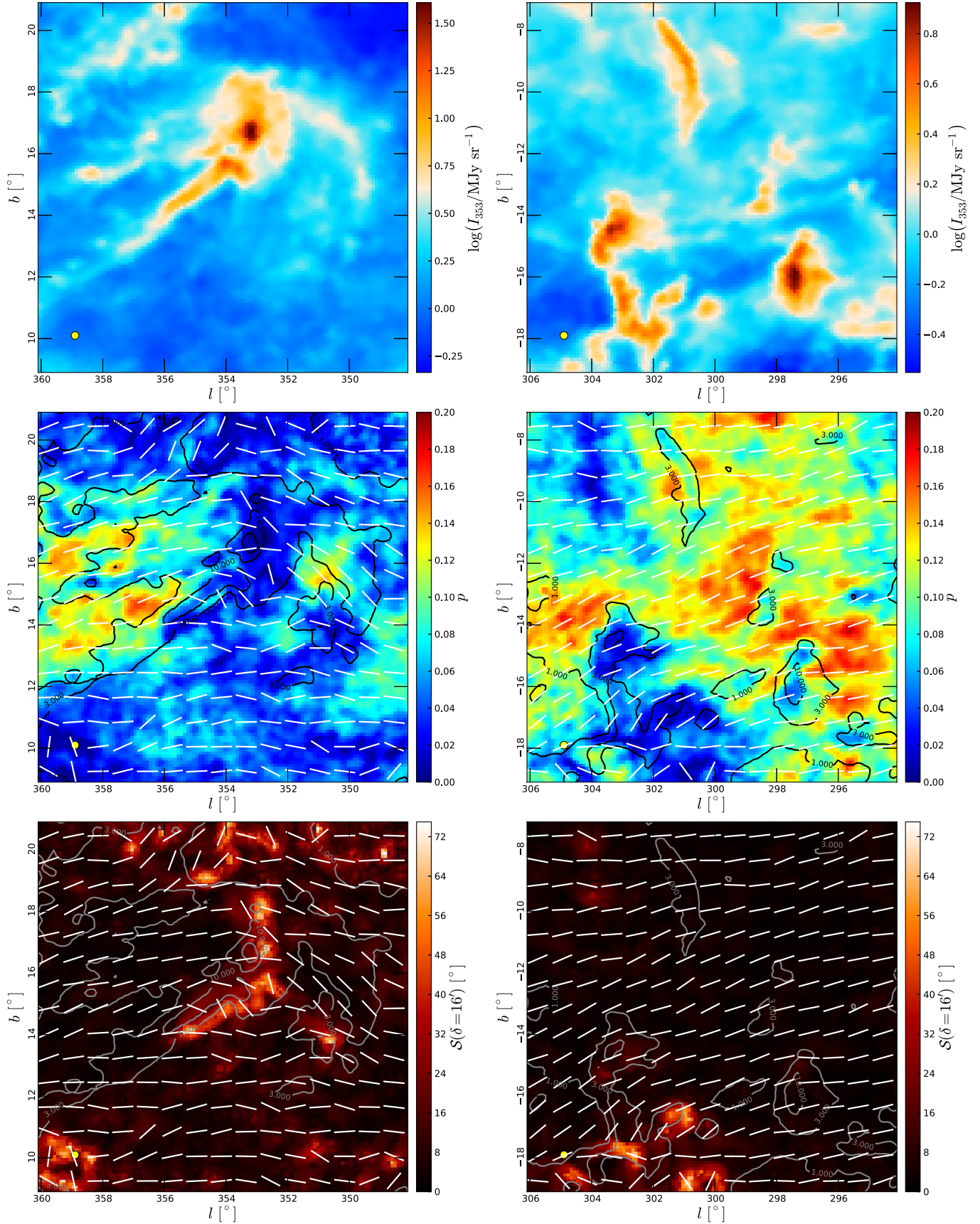
Fig. 3. Maps of the Ophiuchus and Chamaeleon-Musca fields. Left: Ophiuchus field. Right: Chamaeleon-Musca field. Top: total intensity at 353 GHz. Middle: polarization fraction p , column density N_{\text{H}} (contours in units of 10^{21} \text{ cm}^{-2} ), and magnetic orientation (bars, see text). Bottom: angle dispersion function S with lag \delta = 16' (see Sect. 2.5) with contours and bars identical to the middle row. In all maps, the 15' beam is shown in the lower-left corner.
