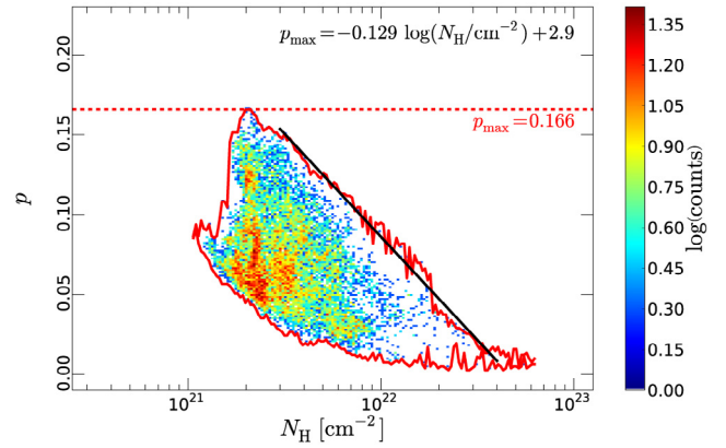
Fig. 5. Same as the top panel of Fig. 4, but using only pixels for which p/\sigma_p > 10 .
