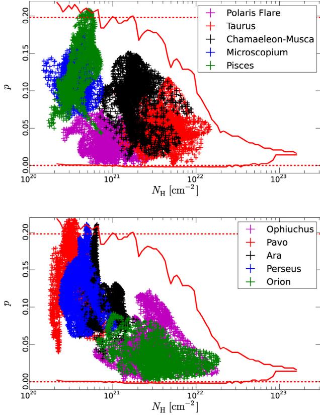
Fig. 2. Two-dimensional distribution functions of polarization fraction p and column density N_H in the fields highlighted in Fig. 1. Top: Polaris Flare (magenta), Taurus (red), Chamaeleon-Musca (black), Microscopium (blue), and Pisces (green). Bottom: Ophiuchus (magenta), Pavo (red), Ara (black), Perseus (blue), and Orion (green). On both panels, the solid red lines show the upper and lower envelopes (see text) of the large-scale distribution of p and N_H , clipped below N_H = 2 \times 10^{20} \text{ cm}^{-2} , while the dashed red lines correspond to p = 0 and the maximum value p = 0.198 (i.e., 19.8%) quoted in Planck Collaboration Int. XIX (2014).
