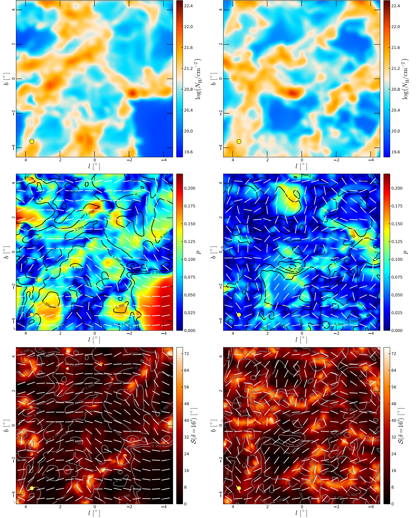
Fig. 15. Simulated Planck maps. Top : total gas column density. Middle : polarization fraction and angle, with contours being the column density at values indicated in units of 10^{21} \text{ cm}^{-2} , and the bars indicate magnetic orientation. Bottom : angle dispersion function at lag \delta = 16' , with the same contours and bars as in the middle row. Left : viewing angle \alpha = 0^\circ . Right : viewing angle \alpha = 90^\circ . In each row, the same colour scale is used. In the lower left corner of each plot (yellow circle) is the 15' FWHM beam.
