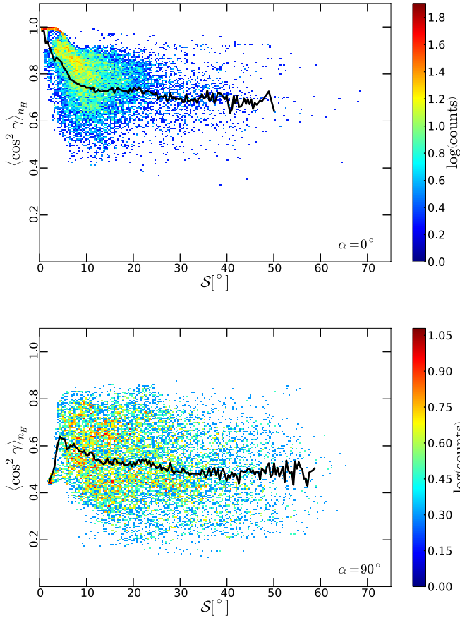
Fig. 24. Distribution functions of angle dispersion function S ( \delta = 16' ) and density-weighted mean of \cos^2 \gamma in the simulation cube. Top : viewing angle \alpha = 0^\circ . Bottom : viewing angle \alpha = 90^\circ . The solid black lines show the mean values per bin of S .
