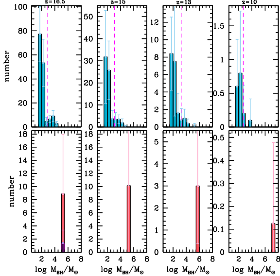
Figure 3. Mass distribution of accreting light (upper panels) and heavy (lower panels) BH seeds at four different redshifts: z = 16.5, 15, 13 , and 10 . The dashed lines in the upper panels indicate the average mass of ILS at the corresponding z .
